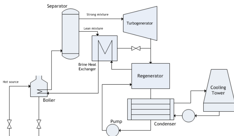
FIGURE 8: KALINA CYCLE HEAT ENGINE
