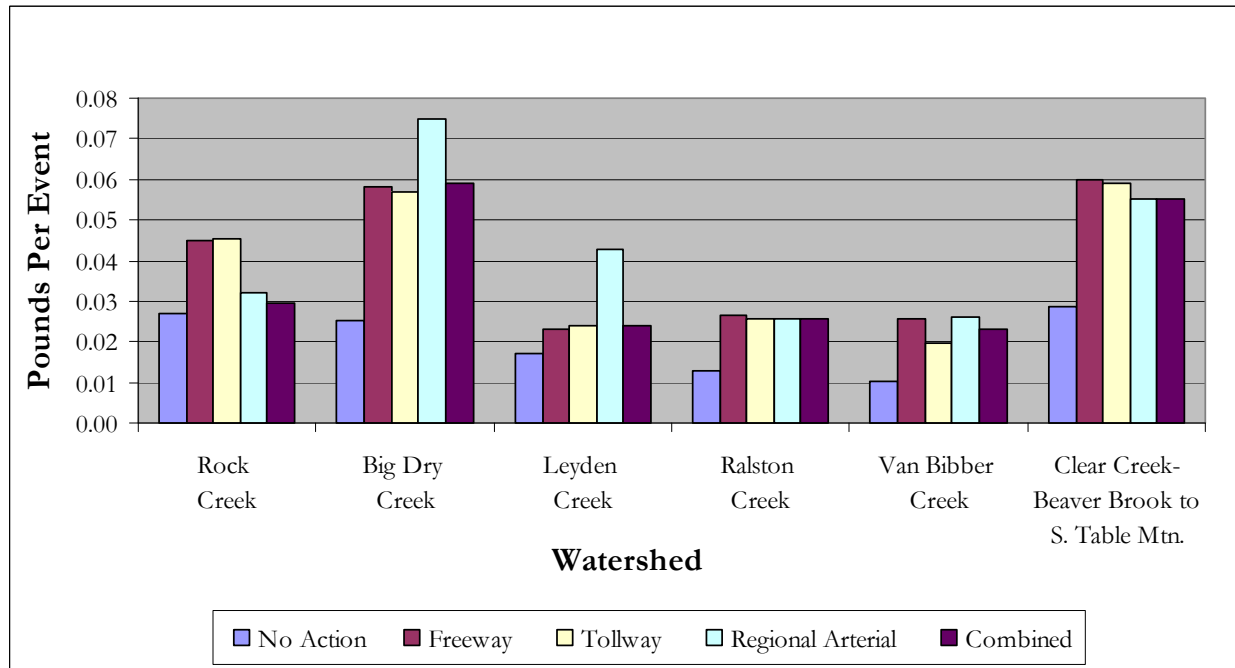
Figure 4.8-6 Copper Loadings along Primary Alignment (US 6 and SH 93)
