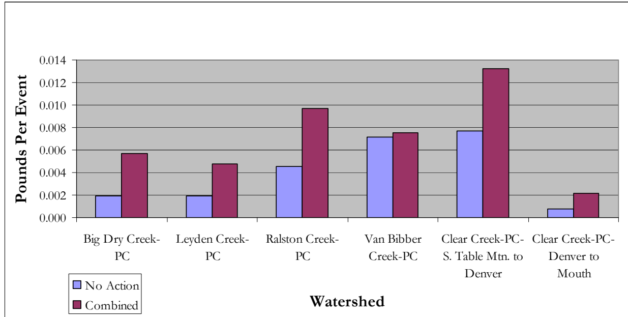
Figure 4.8-8 Total Copper Loadings along Indiana Street/McIntyre Street Alignment
