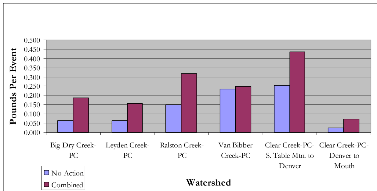
Figure 4.8-9 Total Zinc Loadings along Indiana Street/McIntyre Street Alignment
