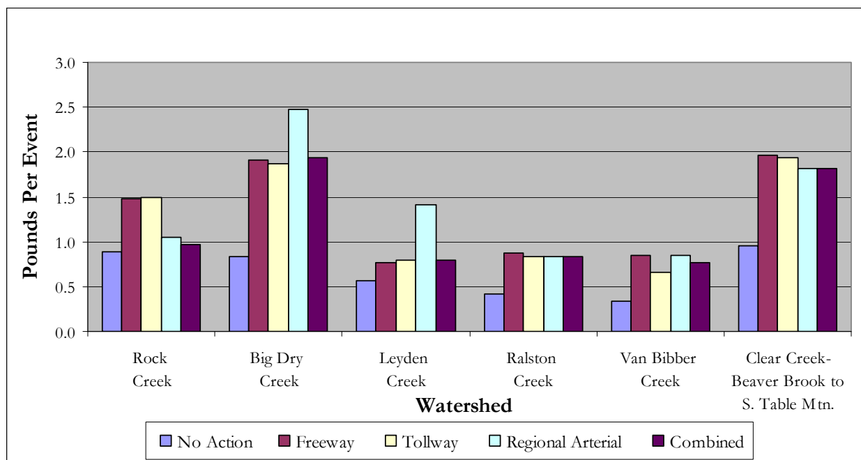
Figure 4.8-7 Total Zinc Loadings along Primary Alignment (US 6 and SH 93)
