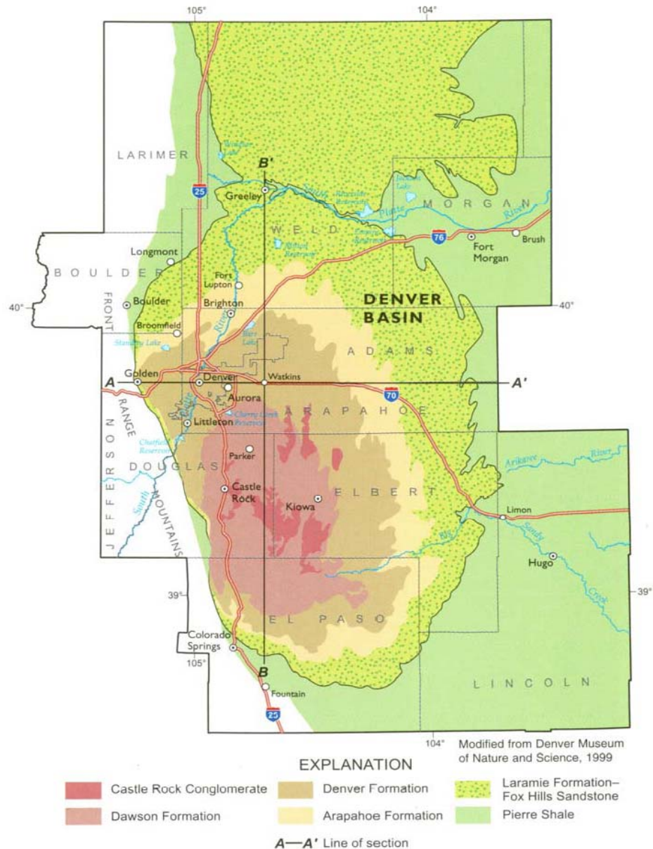
Figure 4.8-5 Generalized Bedrock Geology for the Denver Basin
