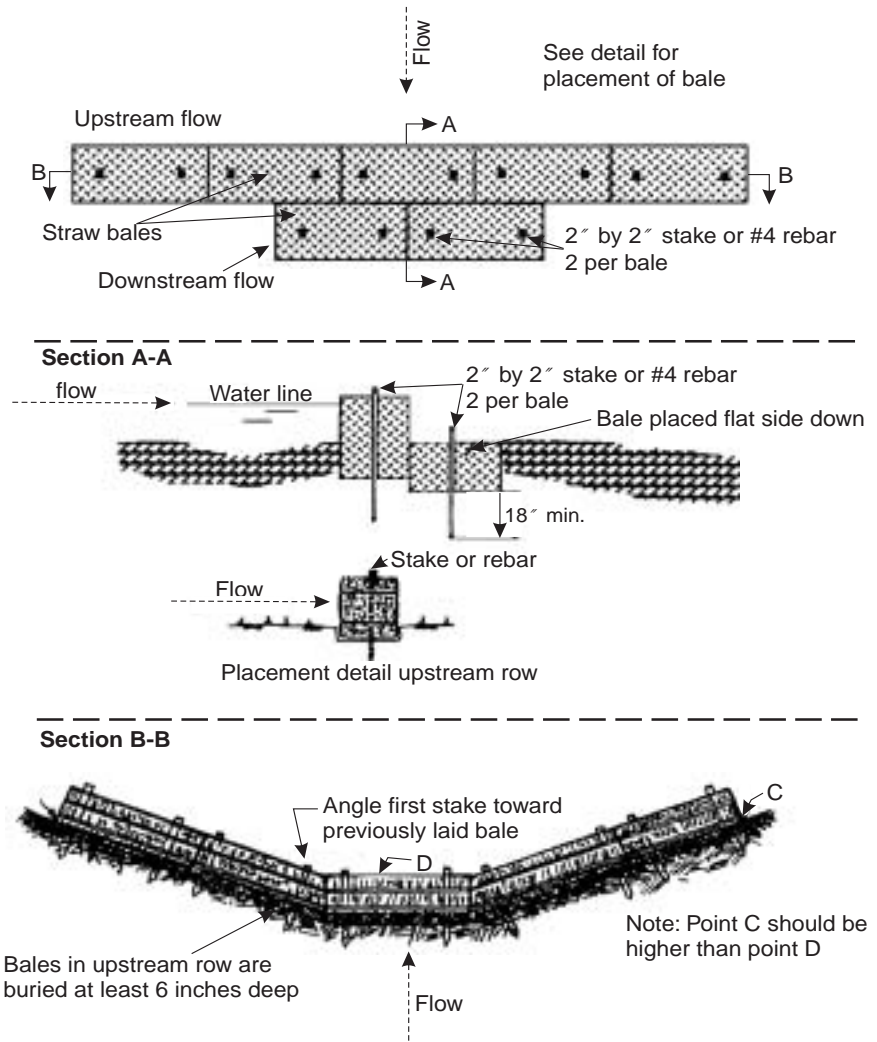
Figure 4. Typical Straw Bale Check Dam
