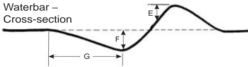
Figure 5. Waterbar construction for forest or ranch roads with little or no traffic. Specifications are average and may be adjusted to conditions.
