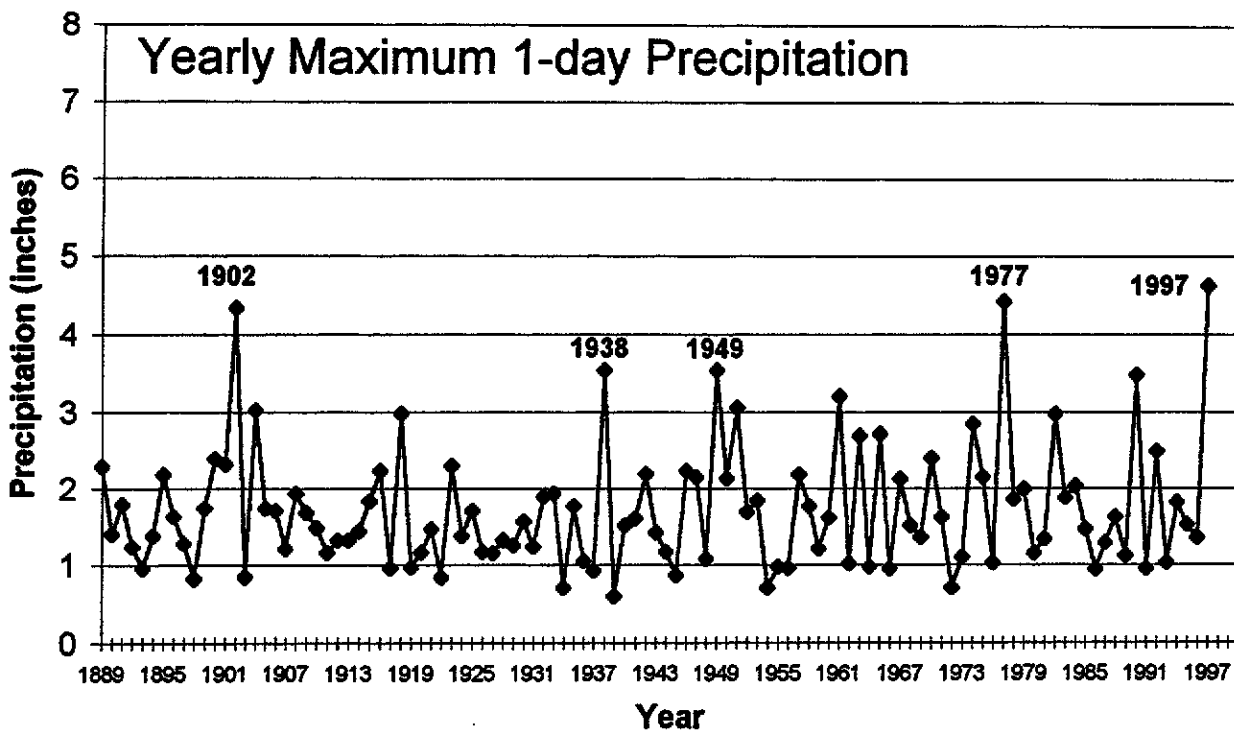
Figure 15. Time series, 1889 through 1997, of the Fort Collins, Colorado, annual maximum one-day precipitation totals (24-hour period ending at 1900 MST) measured on campus.
