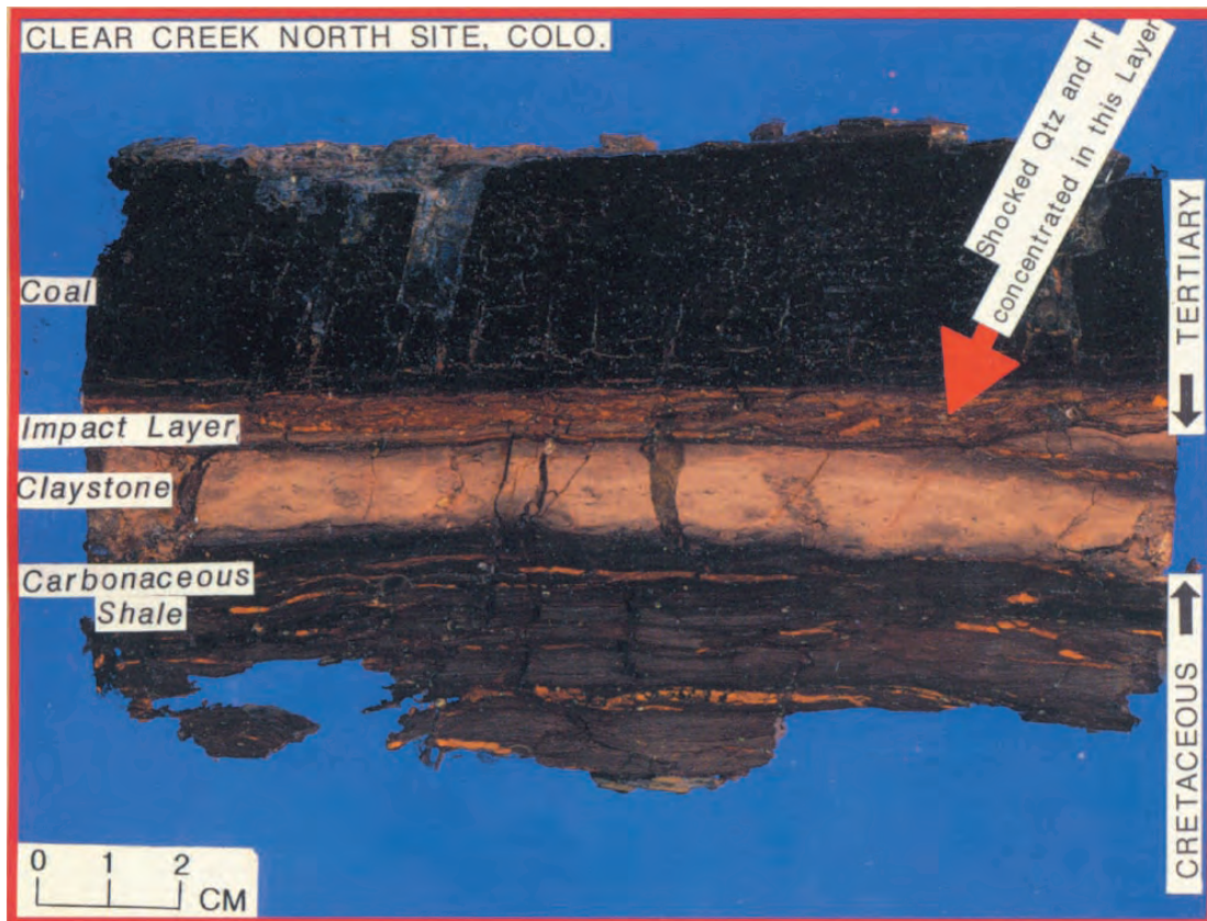
Figure 8. Annotated section of the K/T boundary clay and surrounding beds from the Clear Creek North, Colorado location (from Izett, 1990)
