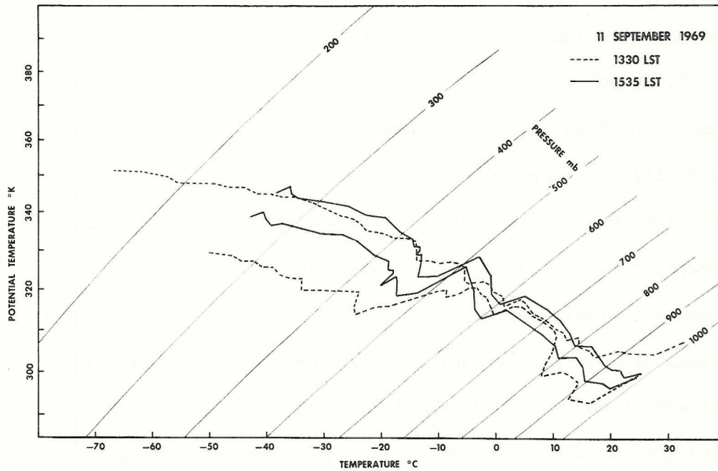
Figure 13. Comparison of atmospheric soundings at Anaco. 11 September 1969.
