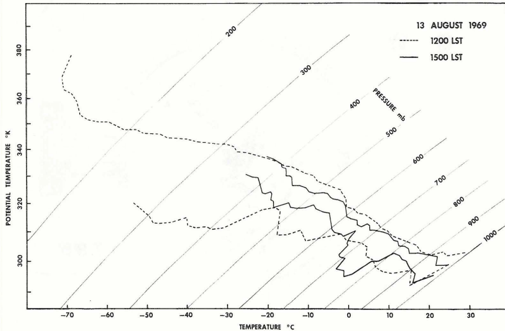
Figure 10. Comparison of atmospheric soundings at Anaco. 13 August 1969.
