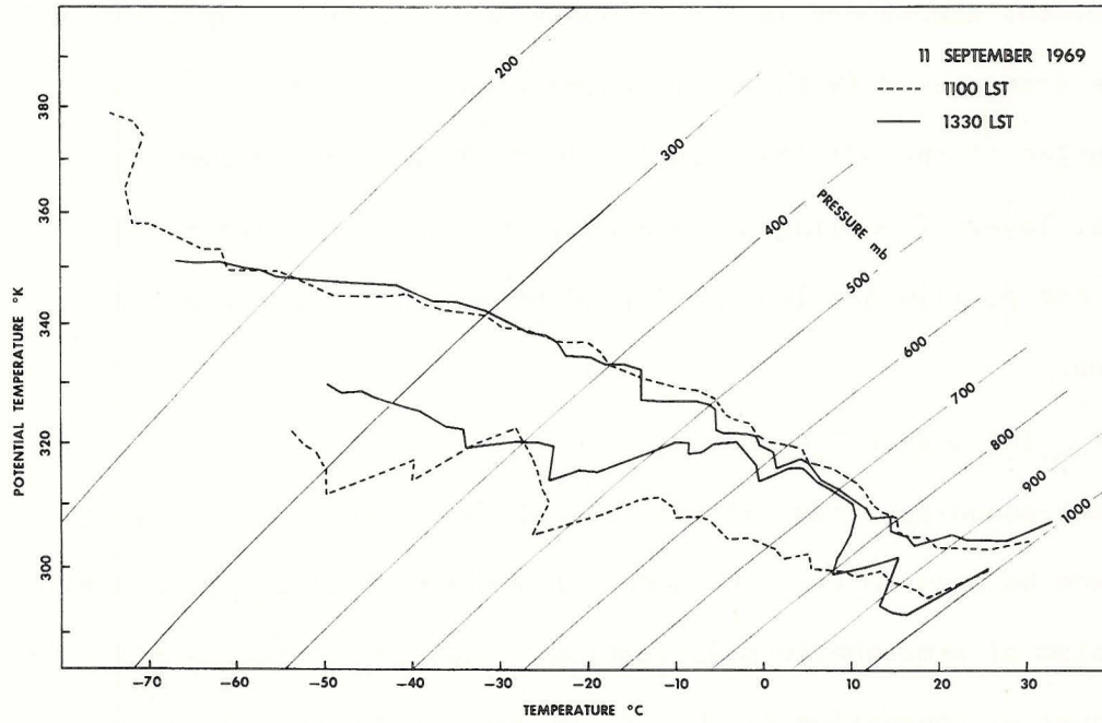
Figure 12. Comparison of atmospheric soundings at Anaco. 11 September 1969.
