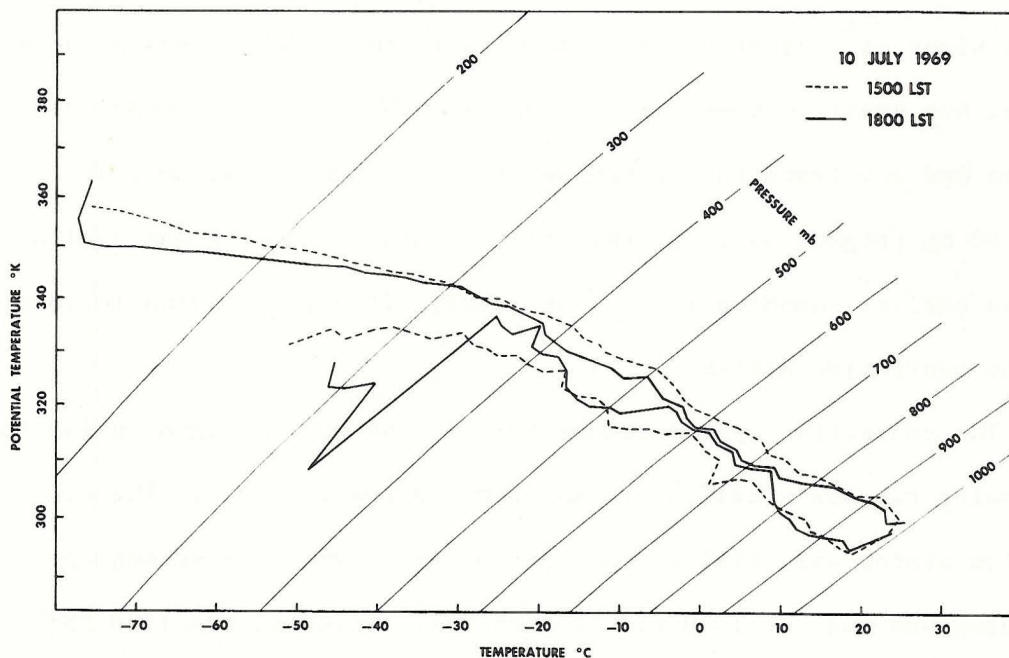
Figure 4. Comparison of atmospheric soundings at Anaco. 10 July 1969.
