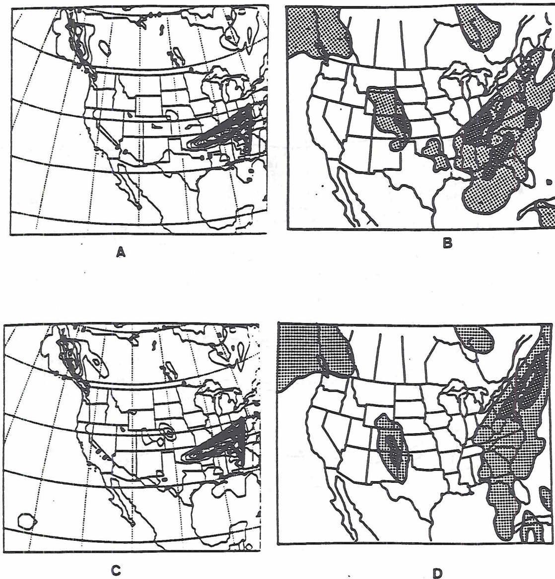
Figure 3.9: (a) RAMS total precipitation at 0000 UTC 30 March, (b) NGM 24-hr forecast for total precipitation (valid 0000 UTC 30 March), (c) RAMS total precipitation at 1200 UTC 30 March, and (d) NGM 36-hr forecast for total precipitation (valid 1200 UTC 30 March). Light stipple 0-1 inches, dark stipple 1-2 inches.
