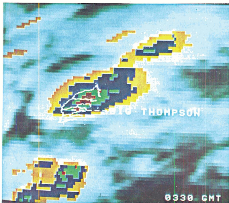
Figure 4-16 Infrared image 1 August 1976 0330 GMT with drainage area overlay.
