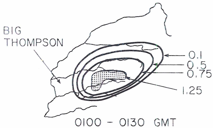
Figure 4-13 Satellite-derived half-hourly isohyet analysis (in), 0100-0130 GMT, 1 August 1976.
