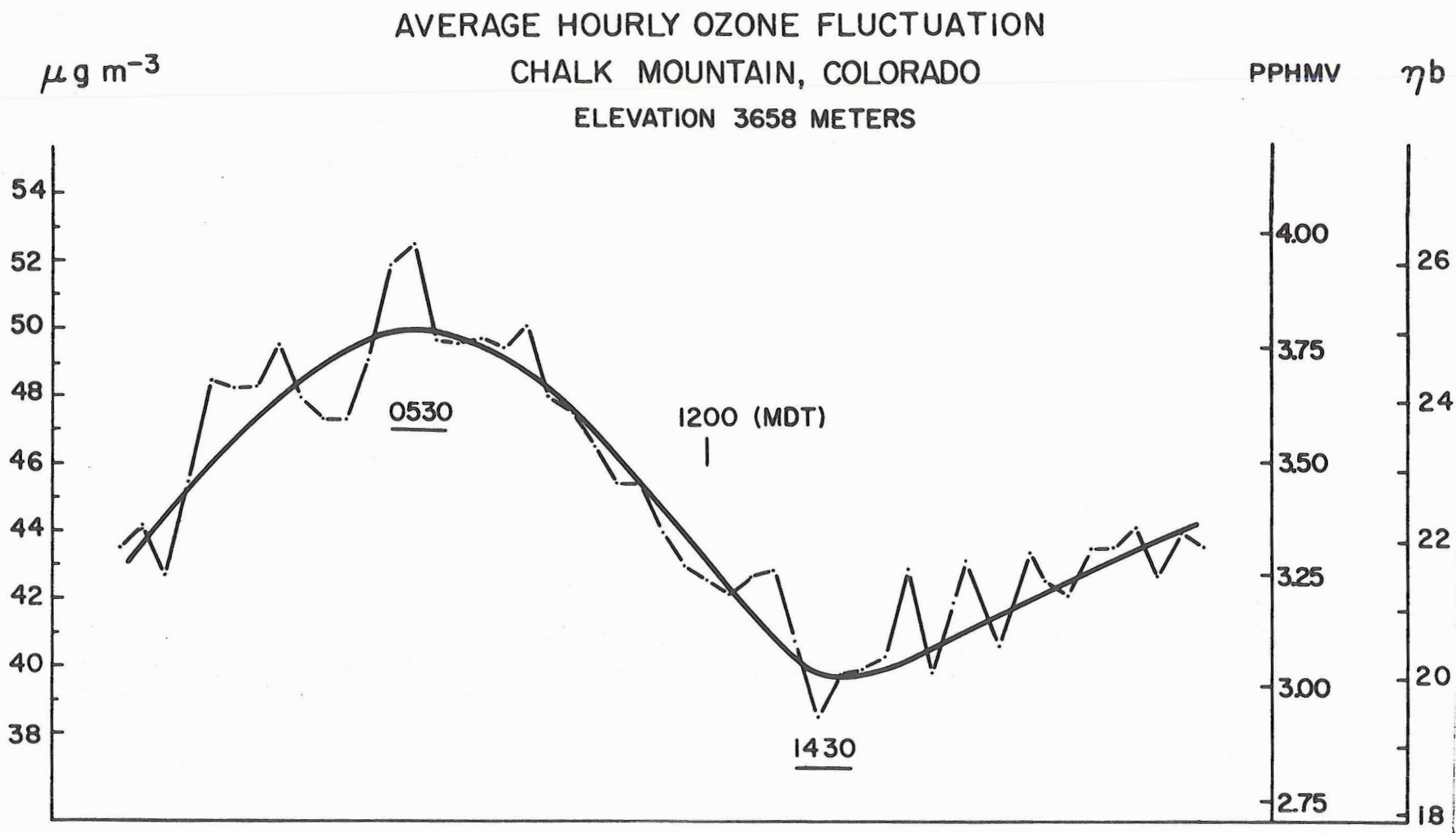
Figure C1. The hourly ozone fluctuation at The Chalk Mountain Observatory. The solid line is a best fit curve through the data points.
