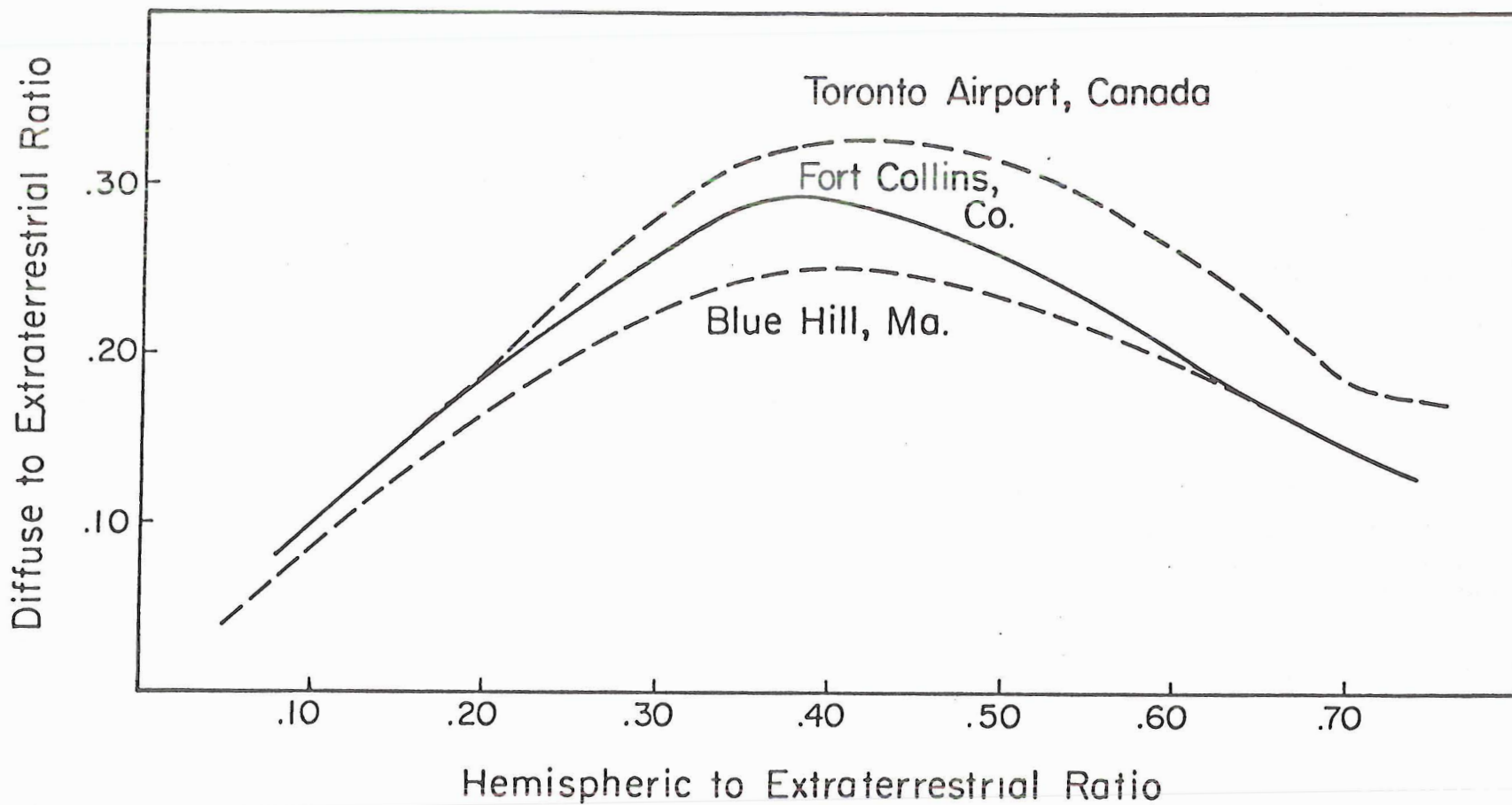
Figure 3. Comparison of the hemispheric/extraterrestrial to diffuse/extraterrestrial correlations of the present study with those of Liu and Jordan (1960) for Blue Hill, MA and Orgill and Hollands (1976) for Toronto Airport, Canada.
