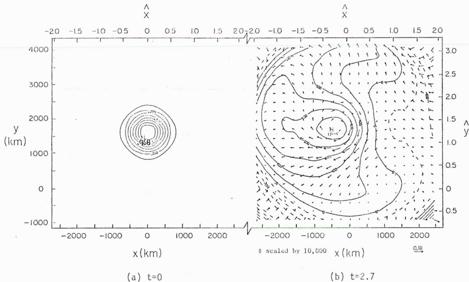
Figure 4.5 Two-dimensional wind and geopotential fields in non-dimensional units for the initial condition of Figure 4.2 at t=0 (a), t=2.7 (b), t=5.3 (c) and t=8.0 (d). The scales on the top and right are non-dimensional and the bottom and left scales are dimensional for \epsilon=500 . For \epsilon=500 the solution is displayed at t=1 day (b), t=2 days (c) and t=3 days (d).
