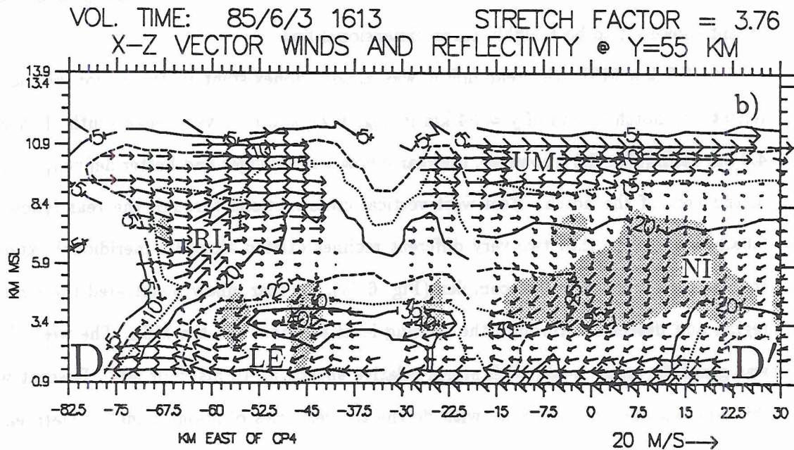
Figure 6.6: Same as in Fig. 6.3 except vertical east-west cross sections of dual-Doppler derived u, w velocities and radar reflectivity in the a) southern rear inflow region ( y = 22 km), b) northern rear inflow region ( y = 55 km), and c) central rear inflow region ( y = 46 km). The labels RI, LE, UM, NI, and SI refer to the Rear Inflow, the Lower level Easterlies, the Upper level wind Maximum, the Northeasterly Inflow, and the Southeasterly Inflow.
