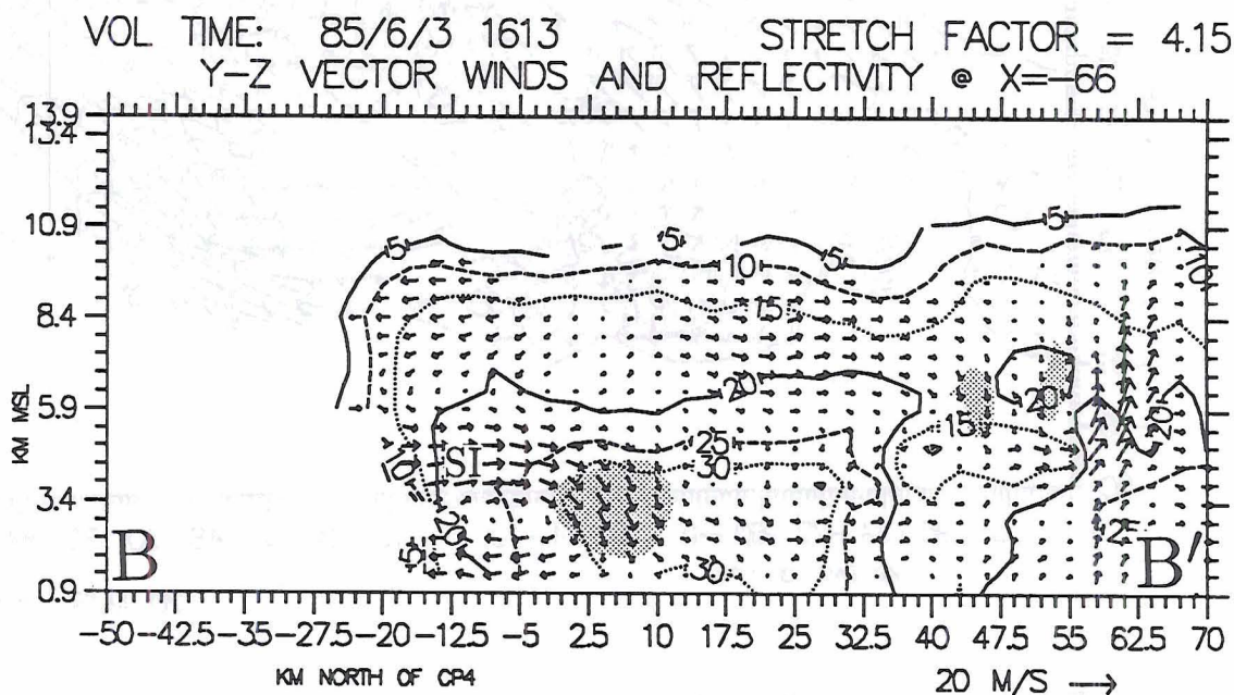
Figure 6.5: Same as in Fig. 6.3, except a vertical cross section corresponding to B-B' at x = -66 \text{ km} in Fig. 6.2.
