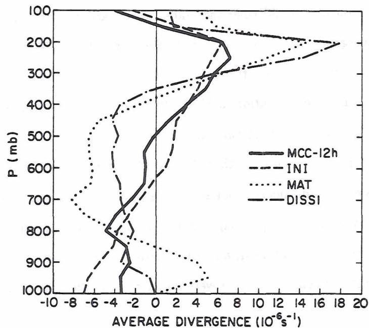
Figure 2.1: Vertical profiles of MCC horizontal divergence (units 10^{-6} \text{ s}^{-1} ) averaged over 4.4 \times 10^5 \text{ km}^2 from Cotton et al. (1989). The lines represent divergence profiles for 12 hrs prior to MCC development, and the MCC initial, mature, and dissipation stages. Profiles were obtained through composites of 90 mid-latitude MCCs.
