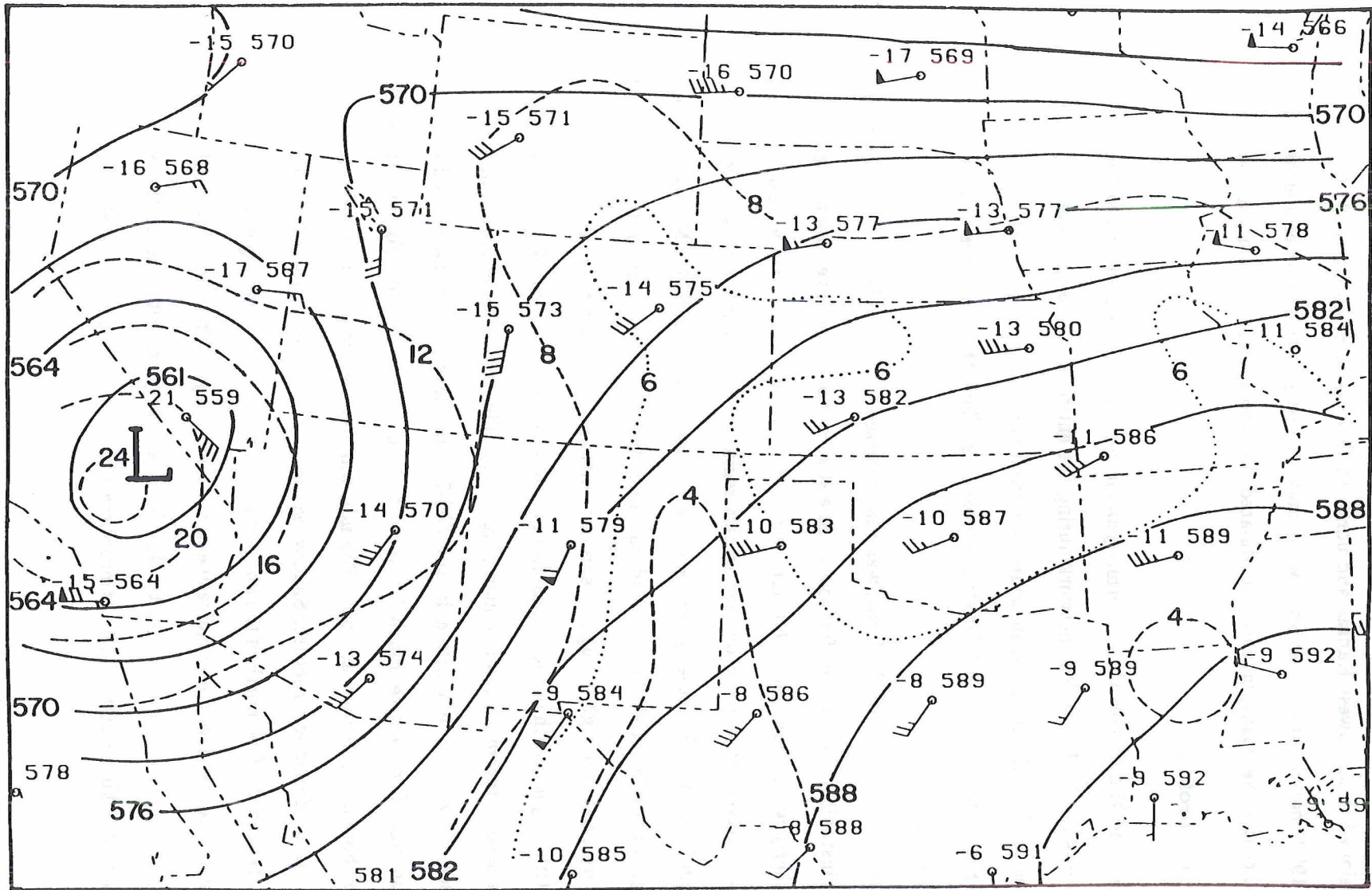
Figure 4.3: The 1200 3 June 500 mb analysis from Fortune et al. (1992). Heights are contoured every 30 m (solid), winds are in \text{ms}^{-1} (one full barb equivalent to 5 \text{ms}^{-1} ), and absolute vorticity every 4 \times 10^{-5} \text{s}^{-1} is contoured starting from 4 \times 10^{-5} \text{s}^{-1} (dash). Note that the 6 \times 10^{-5} vorticity contour has also been added (dot).
