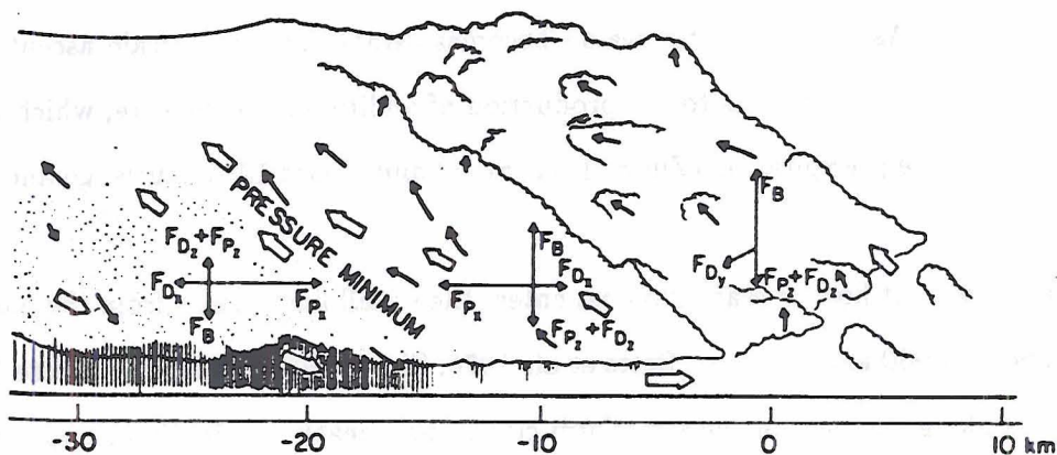
Figure 2.4: Conceptual drawing of a tropical squall line with highly tilted convective updrafts (after LeMone, 1983). F_P , F_D and F_B represent mesoscale pressure gradient, drag and buoyancy forces acting on an air parcel. The location of the pressure minimum responsible for the rear inflow is noted.
