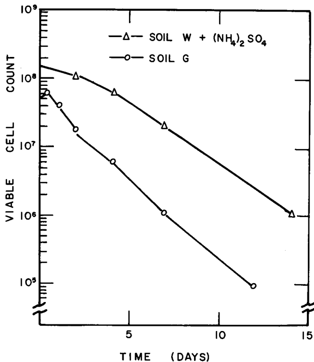
FIG. 5. THE EFFECT ON ESCHERICHIA COLI SURVIVAL IN SOIL W WHEN SULFATE LEVELS WERE RAISED TO THOSE OF SOIL G. (1.32 MG (NH 4 ) 2 SO 4 ADDED TO ONE GM SOIL W. COUNTS BASED ON NUMBER OF BACTERIA PER GM DRY SOIL.)
