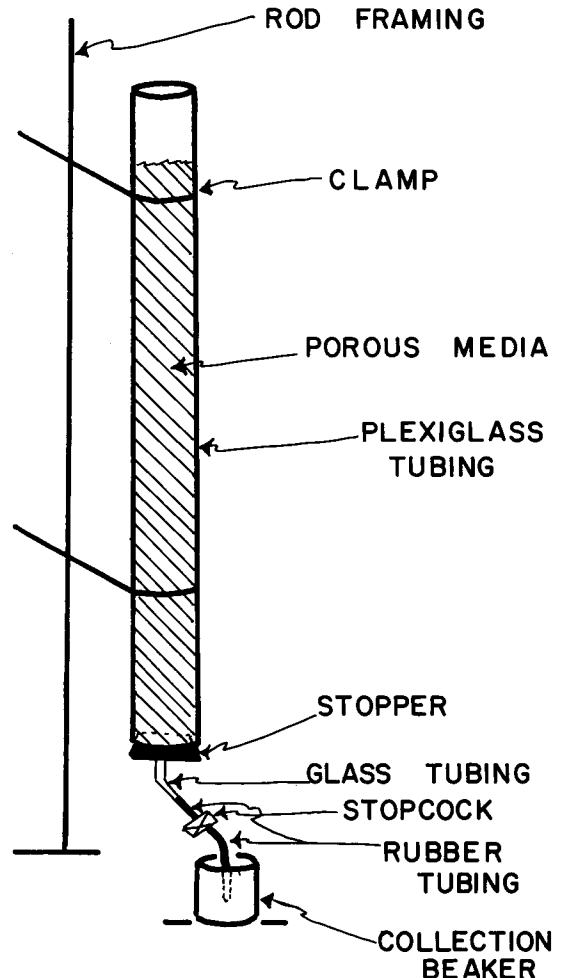
FIG. 9. COLUMN FOR BACTERIAL MOBILITY STUDIES IN POROUS MEDIUM.
