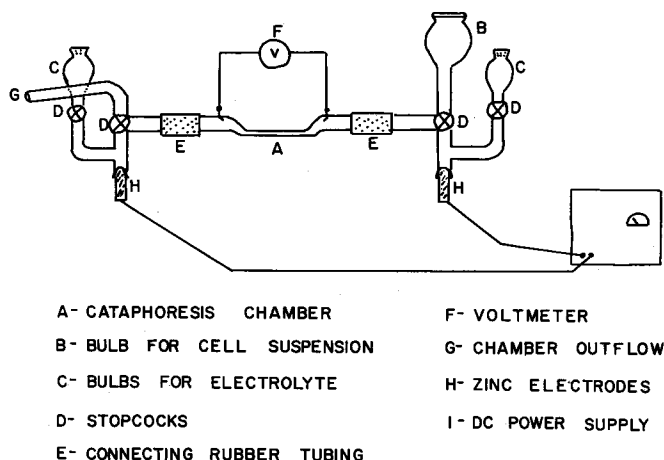
FIG. 10. DIAGRAMMATIC SKETCH OF THE CATAPHORESIS CHAMBER AND ACCESSORY EQUIPMENT.
