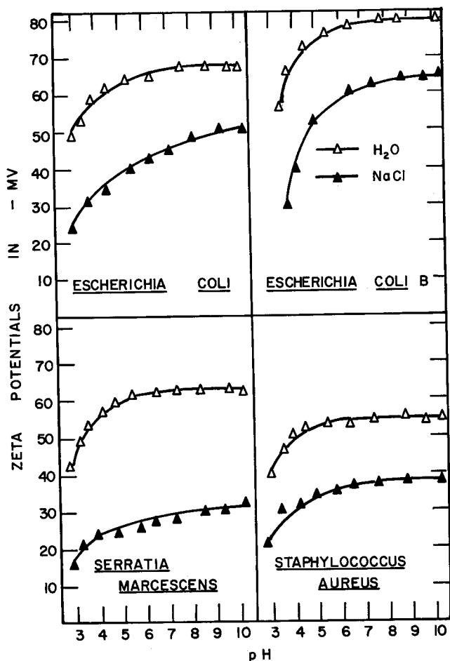
FIG. 11. EFFECT OF PH UPON ZETA POTENTIALS OF FOUR STRAINS OF BACTERIA IN 0.01 N NaCl AND IN DISTILLED WATER.
