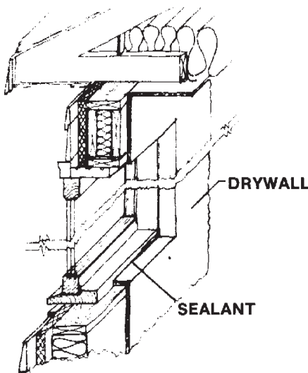
Figure 3: Sealing window openings using the ADA method.
