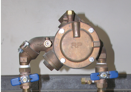
Figure 4: Reduced Pressure Device
