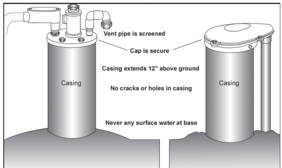
Figure 6. Properly capped and sealed wells protect water quality.
