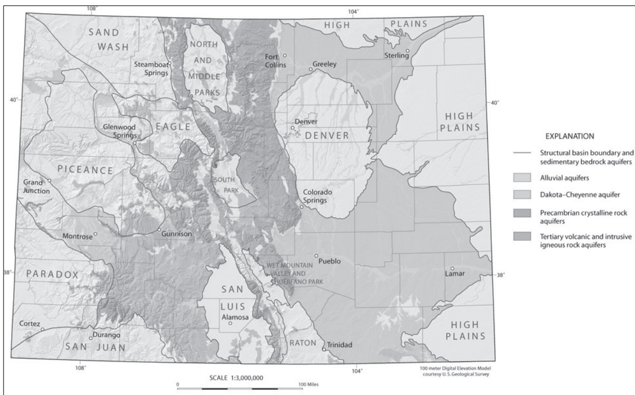
Figure 2. Principle aquifers and basins of Colorado. Source: Colorado Geologic Survey
