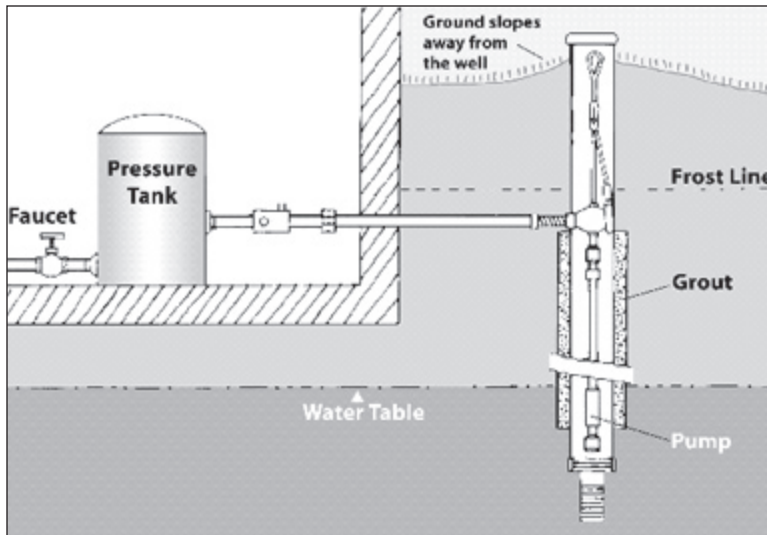
Figure 5. New wells should not have any unsealed openings around the wellhead. Only durable, high quality materials should be used.
