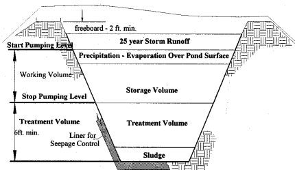
Figure 2 : Waste treatment lagoon.
