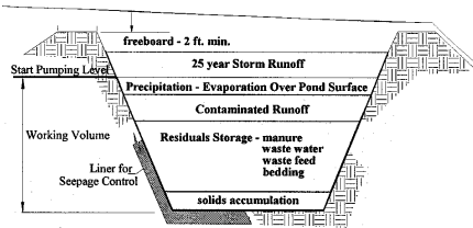
Figure 1: Waste storage pond.
