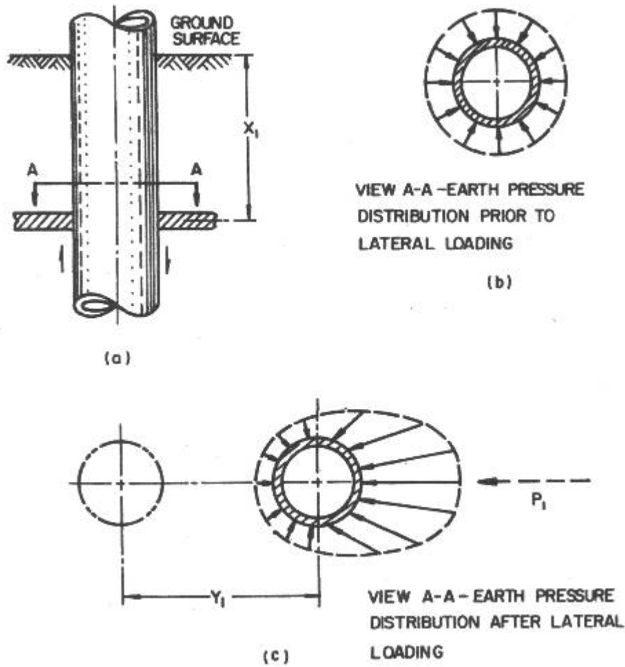
Figure 7-35 Schematic Diagram of p and y (Reese and Allen 1977)
