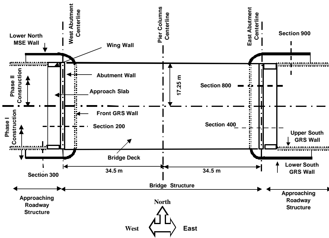
Figure 1.2 Plan View of the Completed Two-span Founders/Meadows Bridge and Approaching Roadway Structures.
