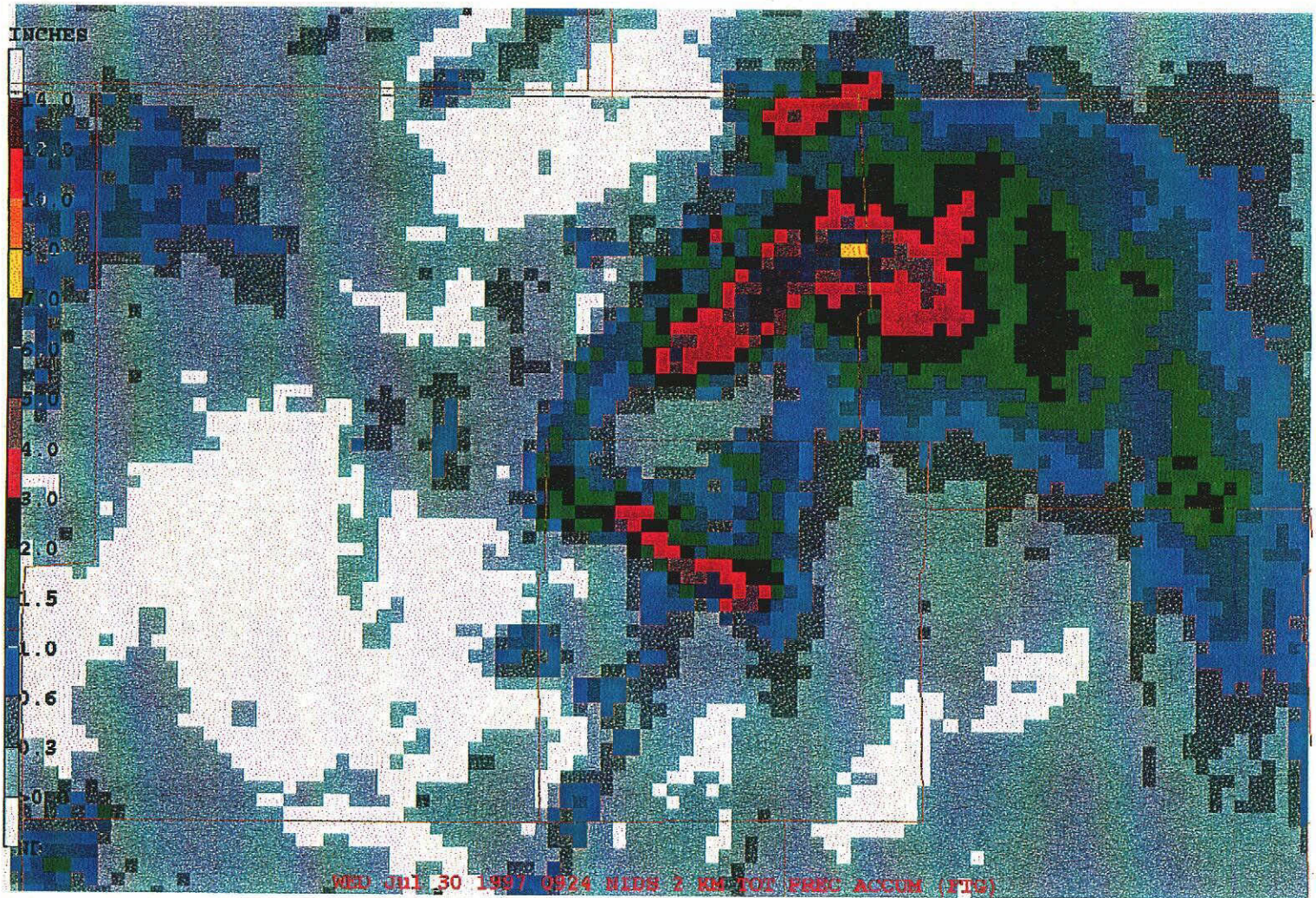
Figure 4. Total precipitation for the period 0000 - 0924Z 30 July 1997.
