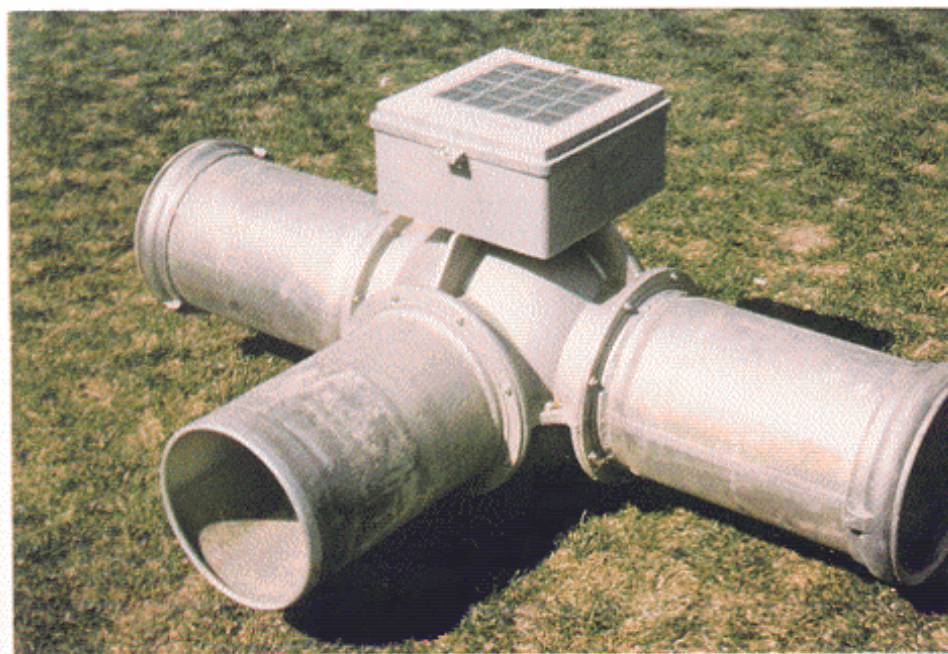
Surge valve. Photo by Grant Cardon, Colorado State University
