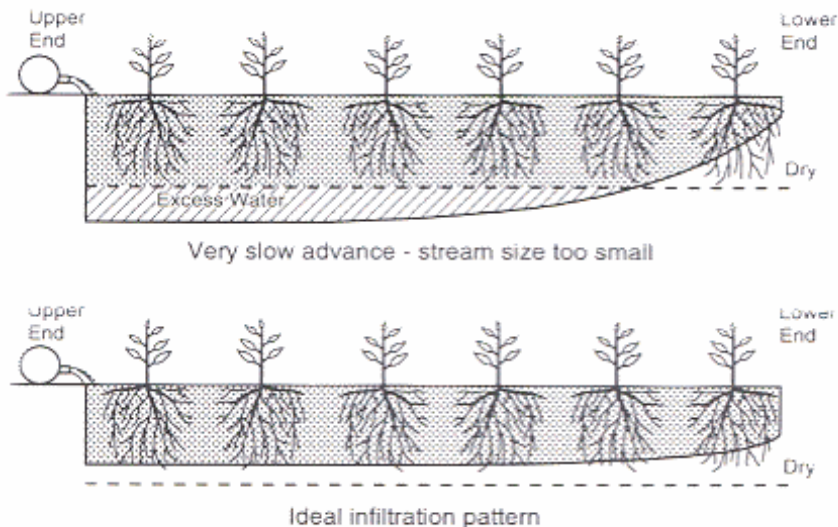
Figure 4. Infiltration patterns with furrow irrigation. Source: Eisenhauer et al., 1991
