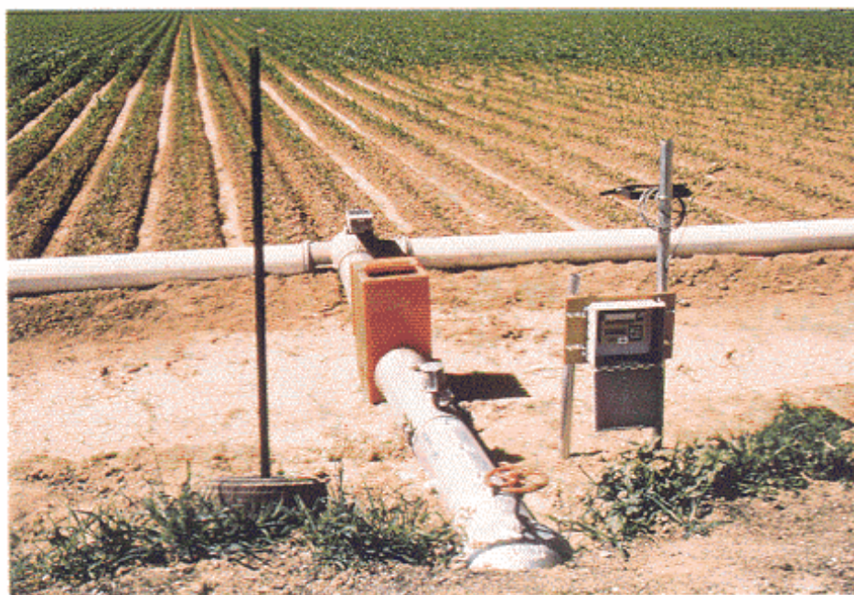
Surge irrigation system. Photo by Grant Cardon, Colorado State University
