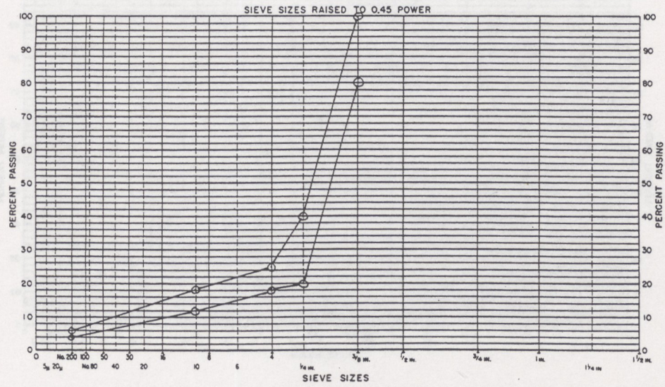
Fig. 5. French Drainage Layer (Course)
