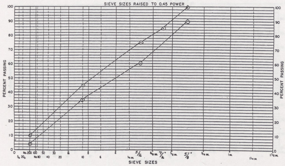
Fig. 6. German Asphalt Concrete (Wearing Course).
