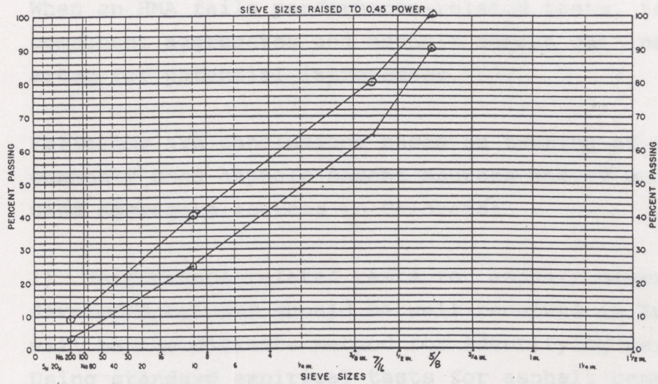
Fig. 8. German Asphalt Binder Course.
