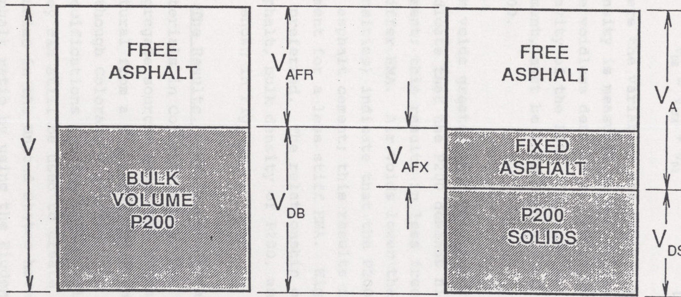
FIG. 1 Definition of Parameters Used to Describe Voids in a P200 and Asphalt Cement Mastic
