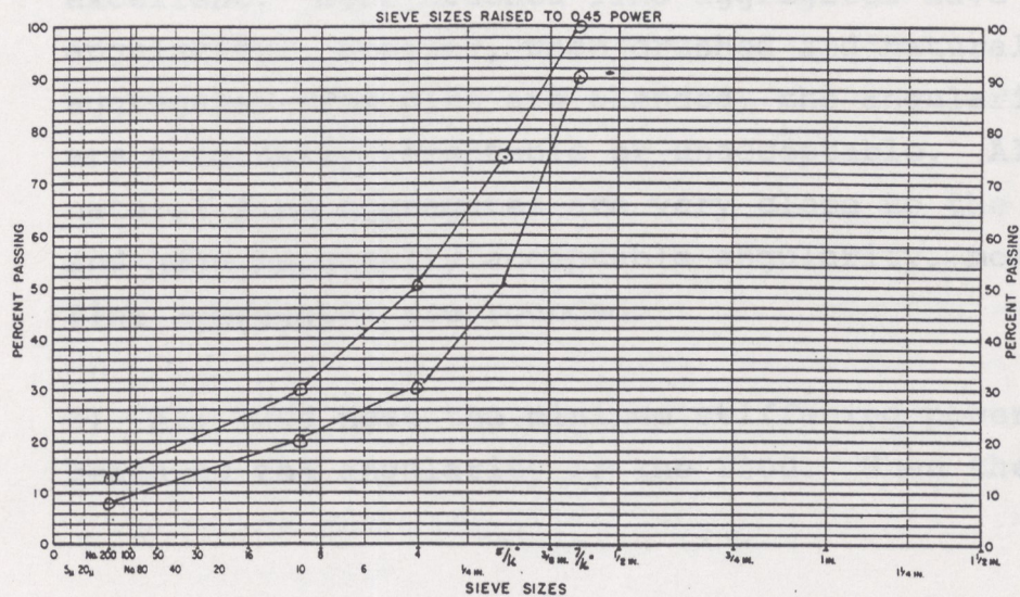
Fig. 9. German Split Mastix Asphalt
