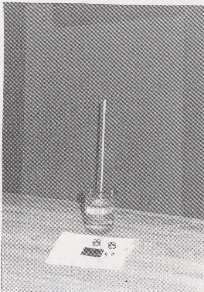
Photo 2. Ring and Ball Equipment Used to Measure Stiffening Effect of P200
