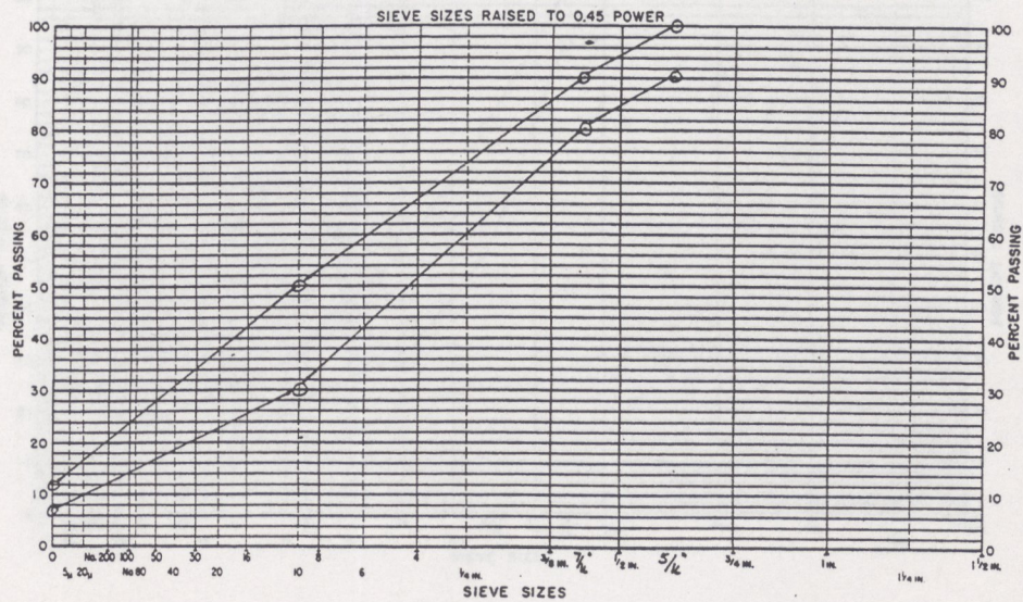
Fig. 7. German All-Purpose HMA.
