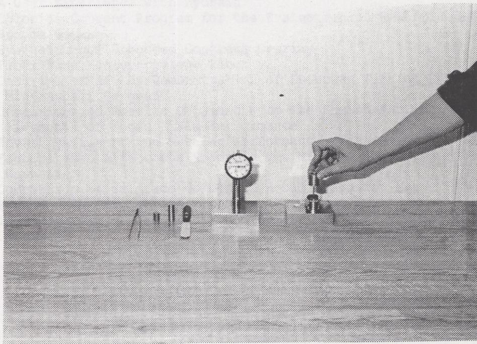
Photo 6. Rigden Voids Index Test Equipment
