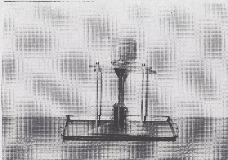
Photo 1. NAA Particle Shape and Texture Test Procedure
