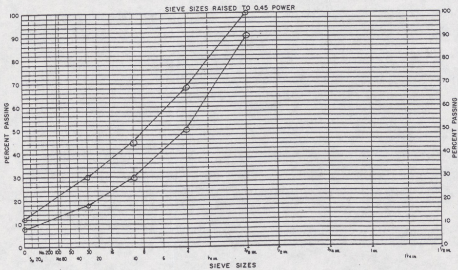
Fig 3. French Classical HMA
