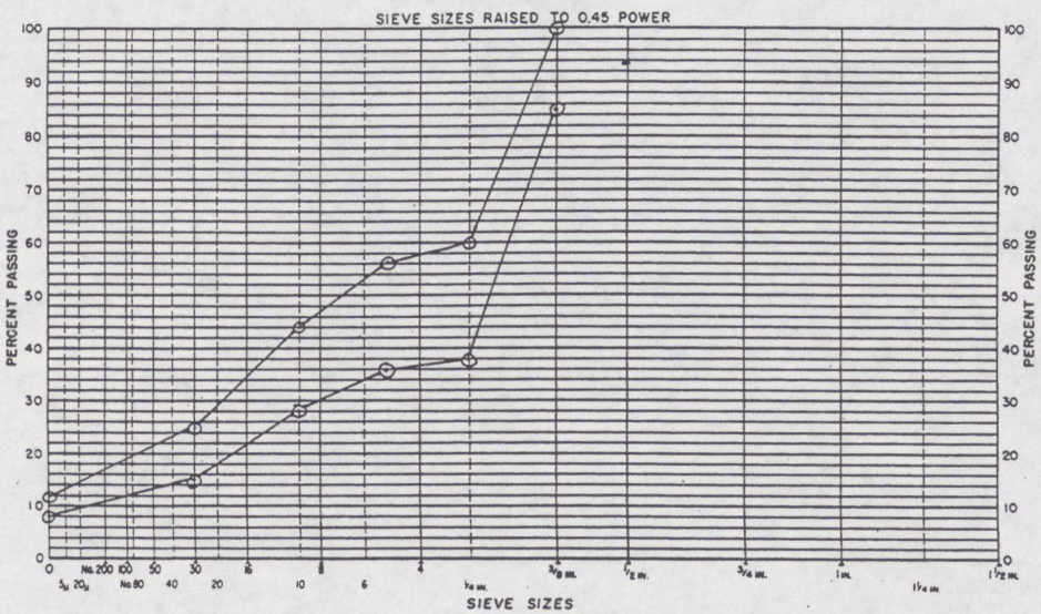
Fig. 4. French Maintenance HMA.
