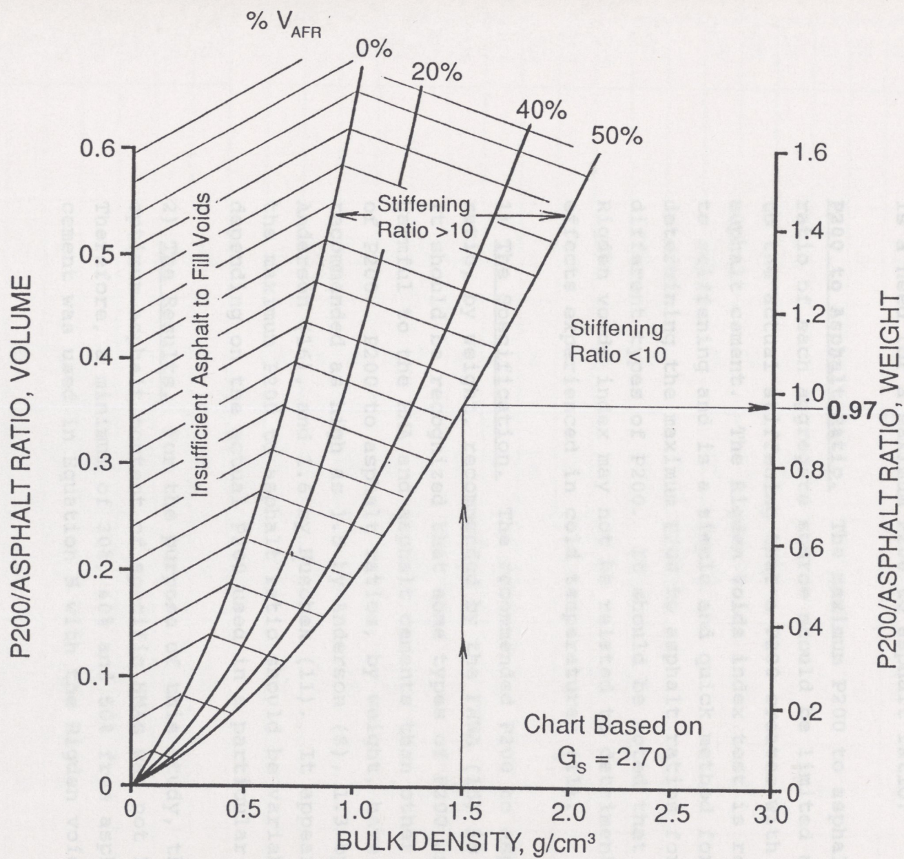
FIG. 2. Design Curves for Controlling Stiffening on Basis of P200 Bulk Density.
