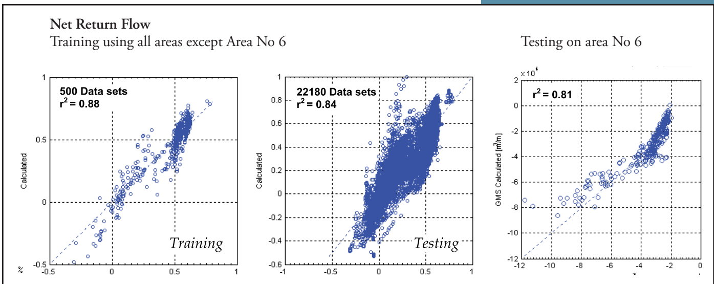
Figure 36. Example of the RB-ANN performance testing outside of the training areas (amended from Triana et al. 2005).
