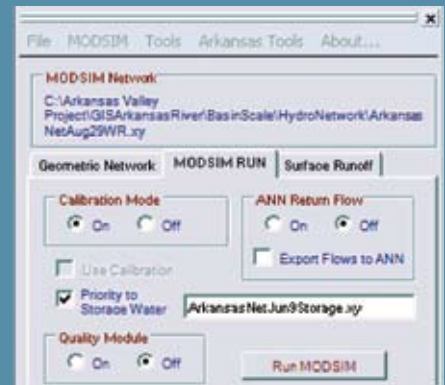
Figure 40. GeoMODSIM running modes interface.
