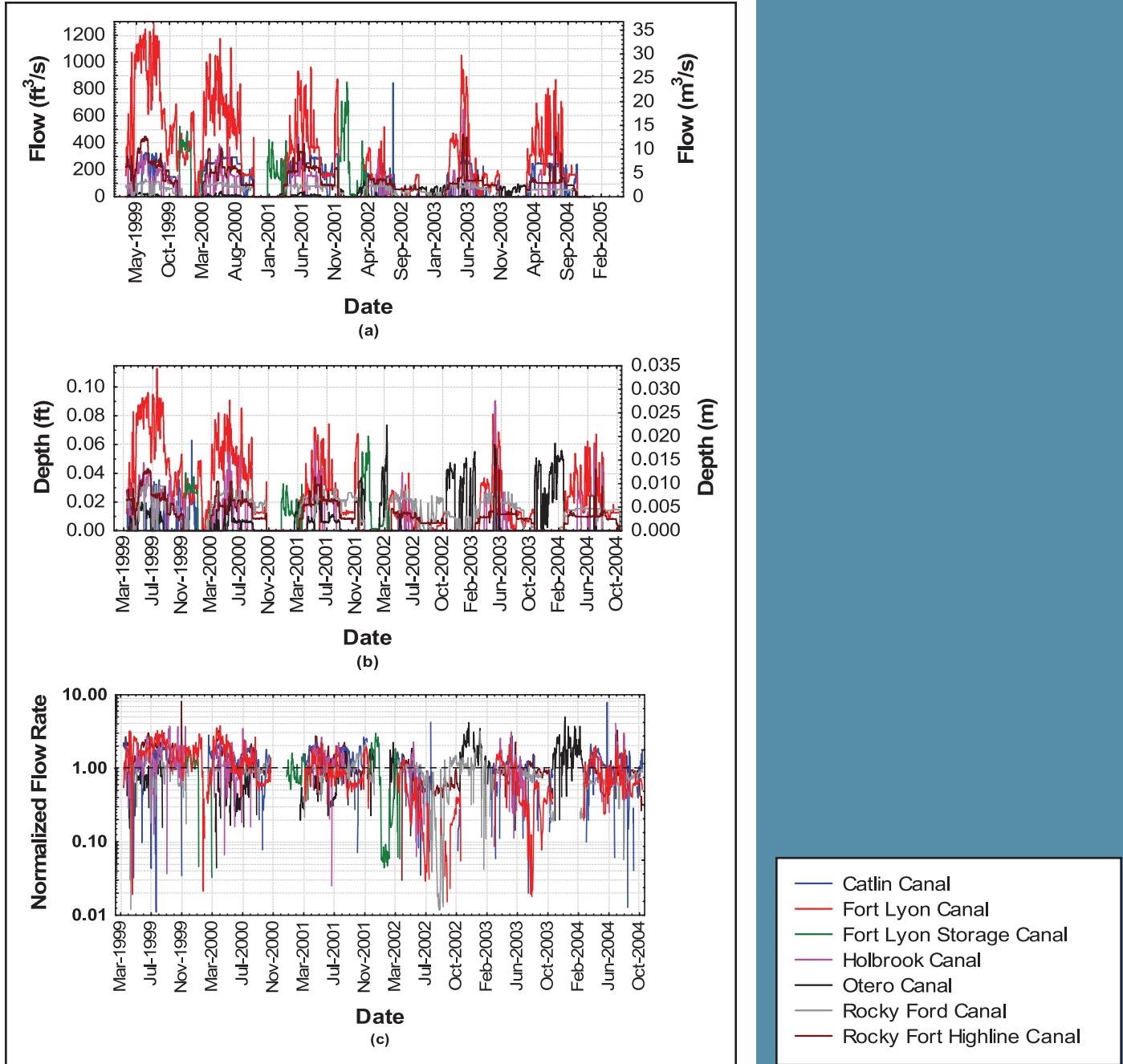
Figure 8. Daily average flow diversions to the major canals in the Upstream Study Region over the period April 1999 – November 2004, expressed as (a) diverted flow rate, (b) flow depth over the entire command area of each respective canal, and (c) ratio of diverted flow rate to mean diverted flow rate over the period 1975 – 2004.
