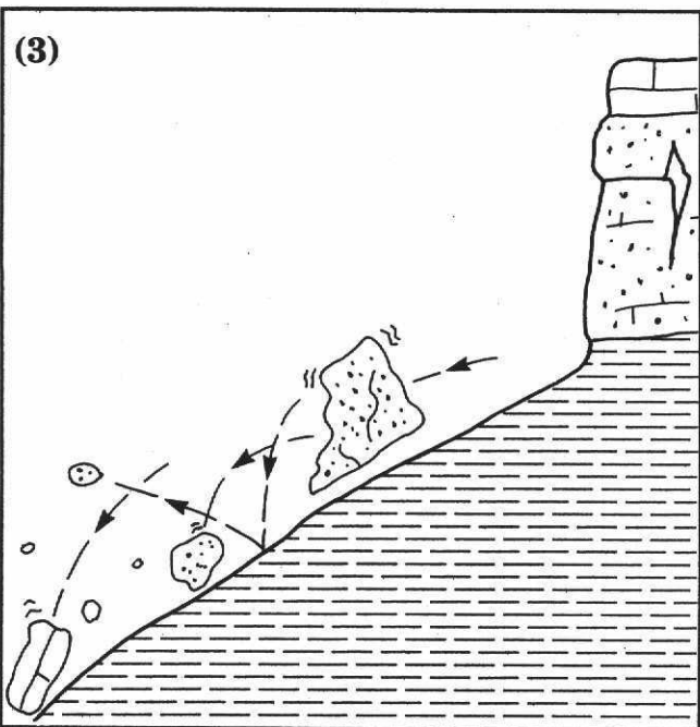
Figure 9a. Topple (Colorado Geological Survey et al., 1988).
