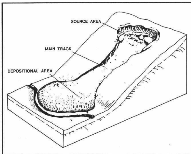
Figure 16a. Earthflow (modified from Varnes, 1978).
