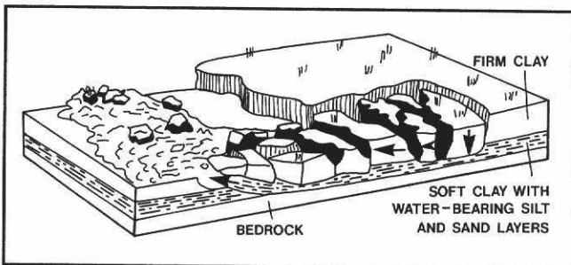
Figure 13a. Lateral spread (Colorado Geological Survey et al., 1988).
