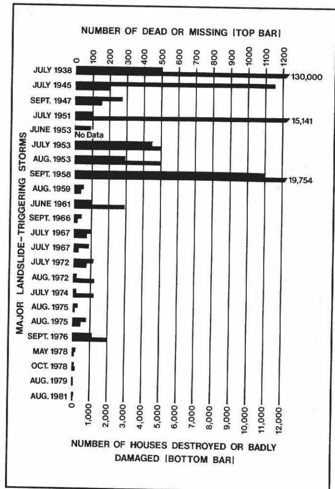
Figure 4. Losses due to major landslide disasters (mainly debris flows) in Japan from 1938–1981. All of these landslides were caused by heavy rainfall, most commonly related to typhoons, and many were associated with catastrophic flooding (data from Ministry of Construction, Japan, 1983).
