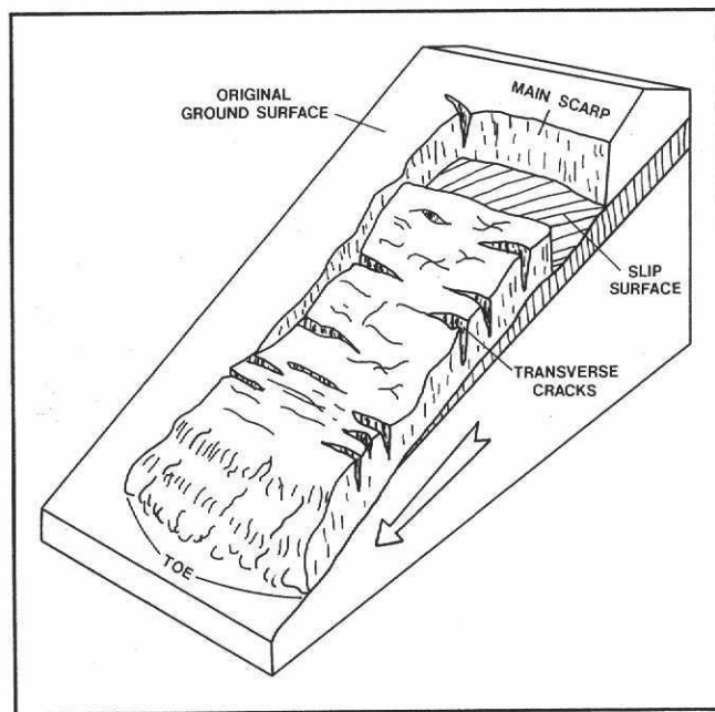
Figure 11. Translational slide (Colorado Geological Survey et al., 1988).
