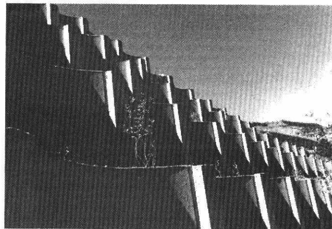
Figure 27. Retaining wall, Interstate 70, near Vail, Colorado (photograph by Colorado Geological Survey).
