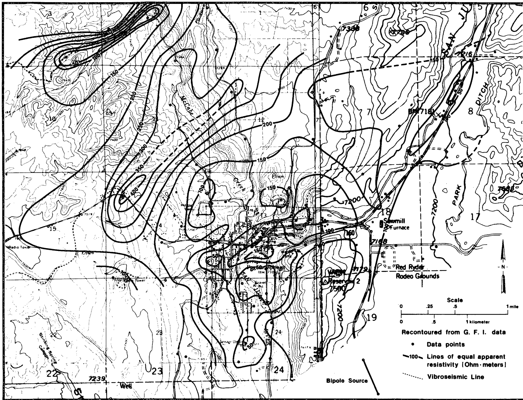
Figure 5 - Dipole - Bipole Resistivity, Pagosa Springs, Colorado
