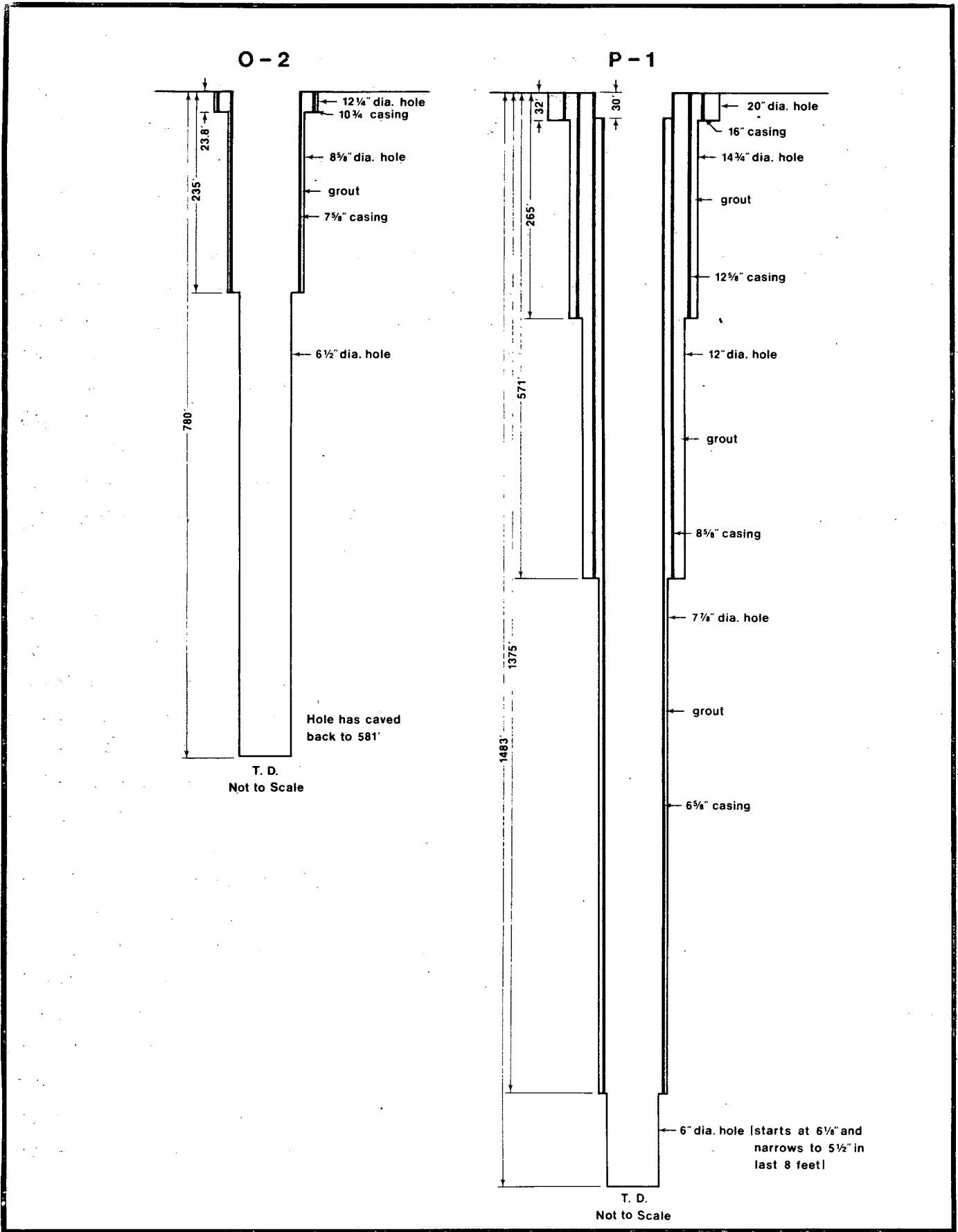
Figure 8 - Well Completion Diagrams of Wells O-2 and P-1
