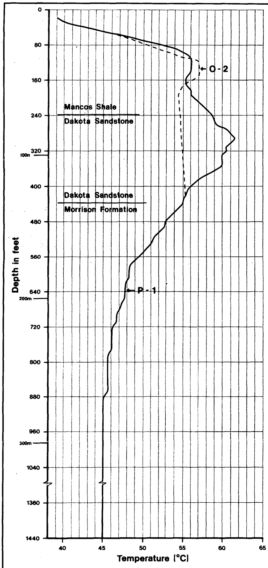
Figure 13 - Temperature Profiles of P-1 and O-2
