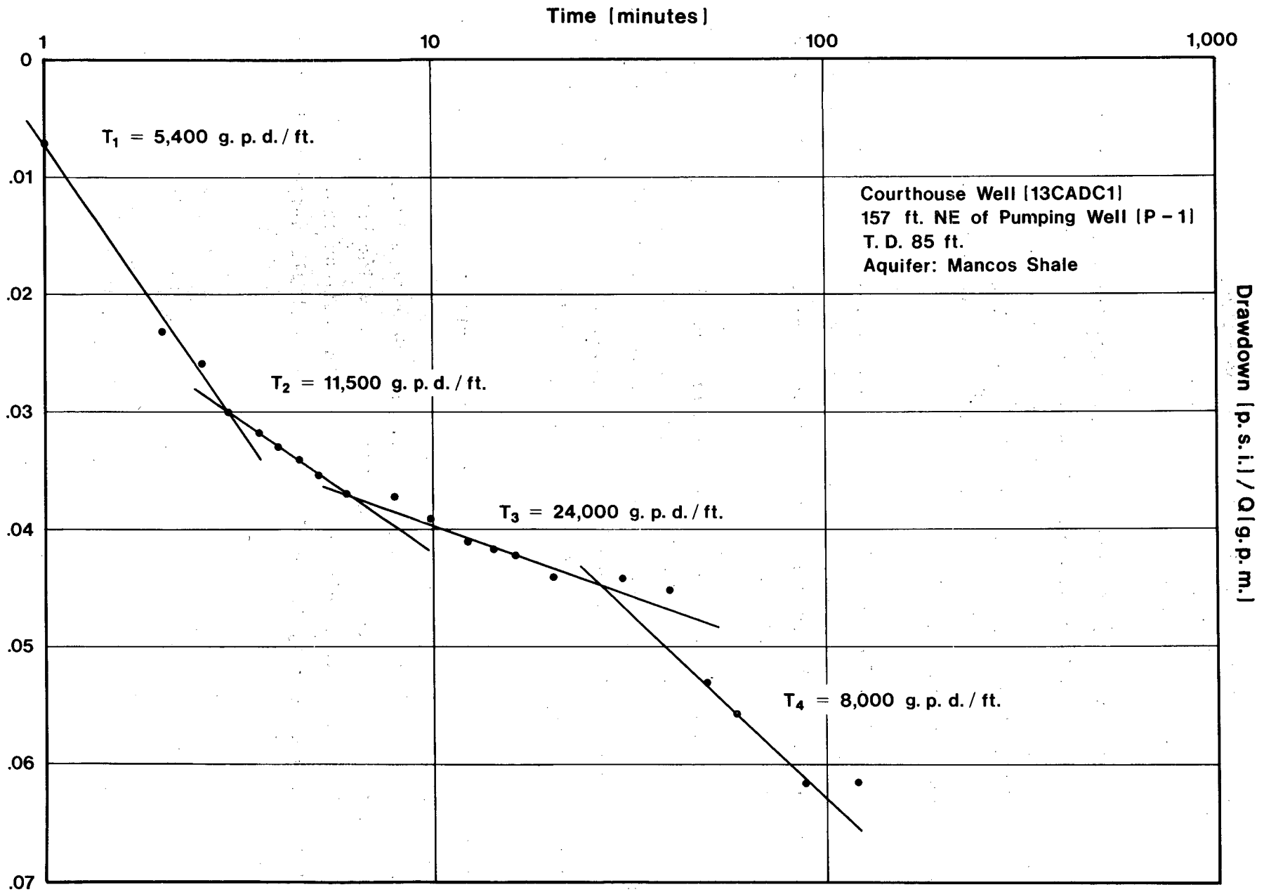
Figure 10 - Time - Drawdown Curve [semi - log] of the Courthouse Well
