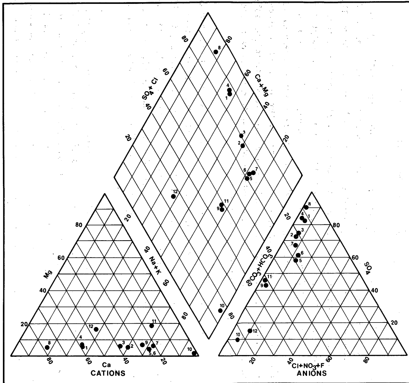
Figure 9 - Trilinear Diagram of Waters from the Pagosa Springs Area
