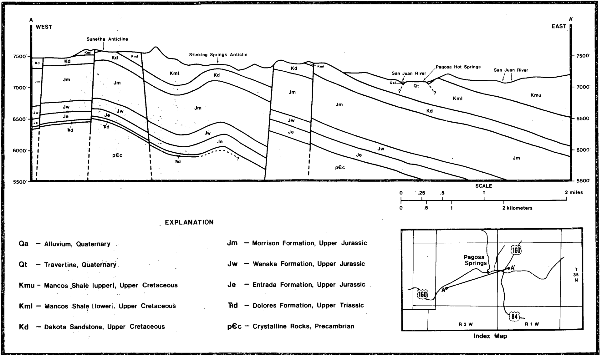
Figure 4 - Cross Section through the Pagosa Springs Area, Colorado
