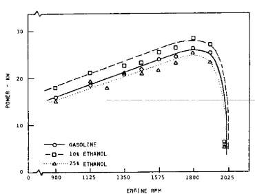
Figure 1. Gasoline engine full throttle power output using ethanol fuel blends.
