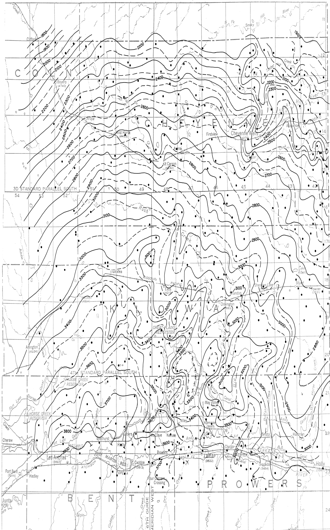
STRUCTURE CONTOUR MAP OF THE TOP OF THE DAKOTA AQUIFER IN THE CHEYENNE WELLS-ANIMAS REGION, COLORADO
