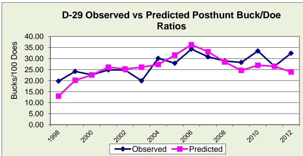
Figure 7. Observed and modeled posthunt sex ratios from 1998 to 2012 for the Mesa Verde Deer Herd.
