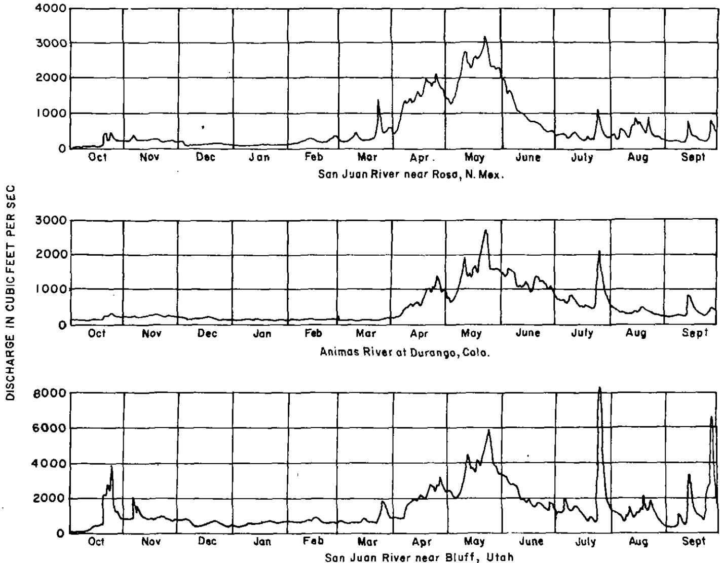
Figure III-2. - Seasonal pattern of runoff of streams in the San Juan River Basin, 1954 water year. Source: USGS Professional Paper 441
