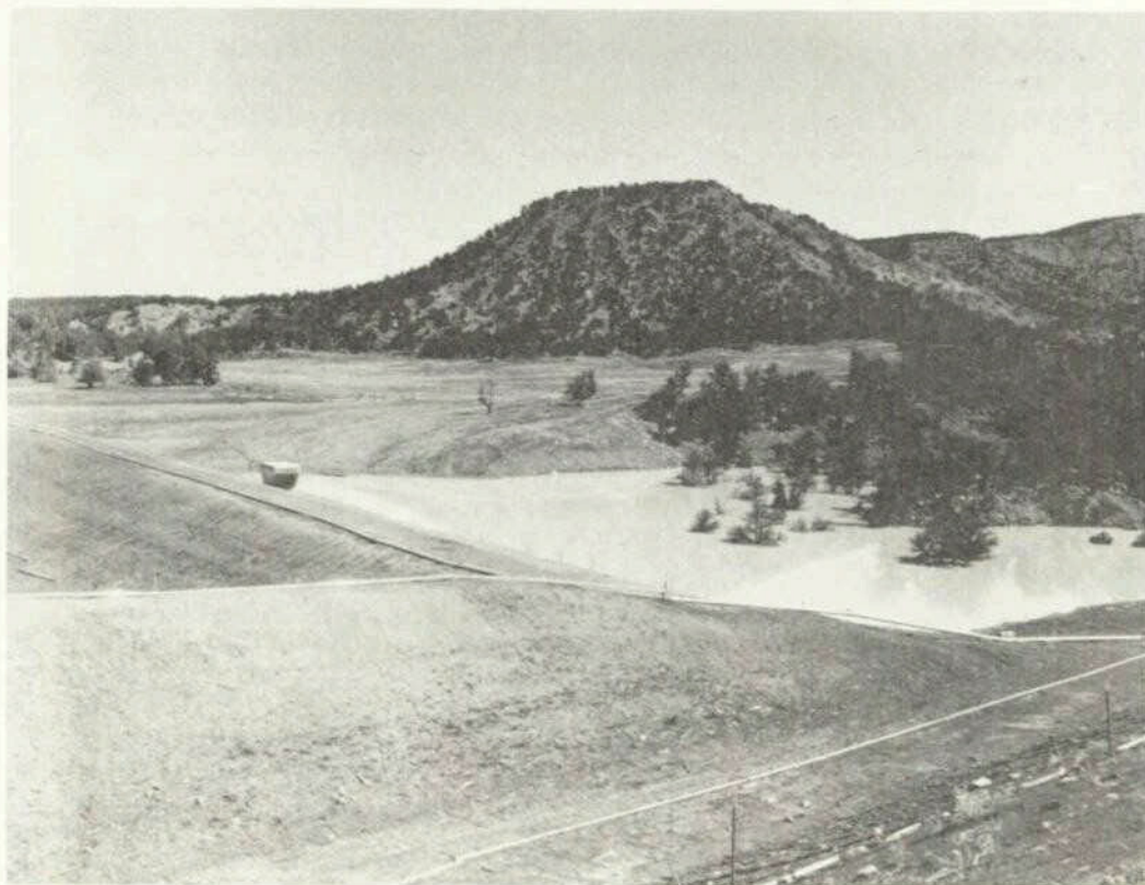
Public Law-566 Floodwater Retarding Structure Pine River Watershed Project, Colorado
