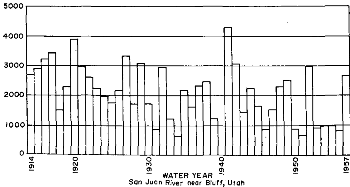
Fig. III-3. Variability of annual discharges of streams in the San Juan River Basin, water years 1914-57.
