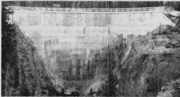
PHOTO 11.2-1 ALKALI-AGGREGATE REACTION. Note typical cracking pattern of exposed concrete.
