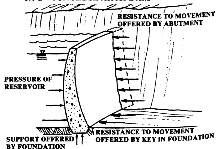
FIGURE 3.6-3 — CONCRETE ARCH DAM
