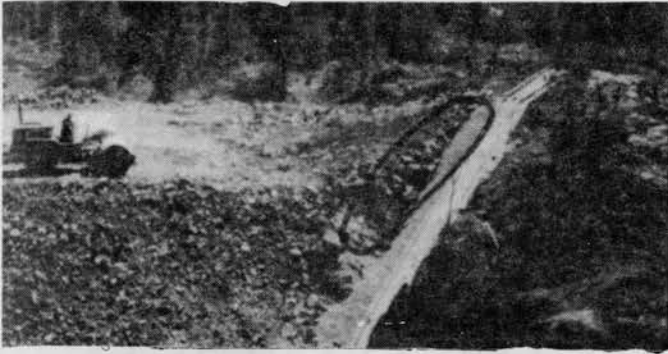
FIGURE 2.5-11 — VIBRATORY ROLLER. Drums vibrate as roller moves.
