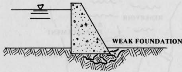
(a) Concrete gravity dam built on a weak foundation.
