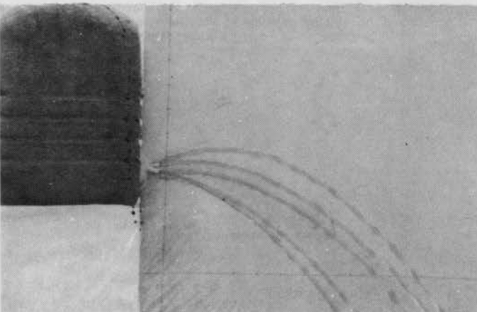
FIGURE 2.8-2 WATER PRESSURE AT ANY POINT ACTS IN ALL DIRECTIONS
