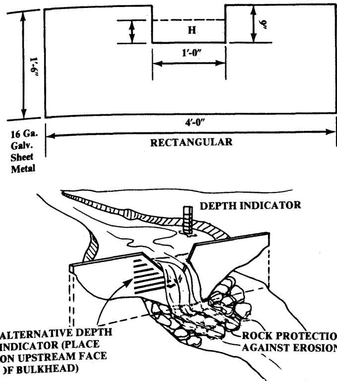
FIGURE 12.4-6 — TYPICAL V-NOTCH WEIR INSTALLATION
