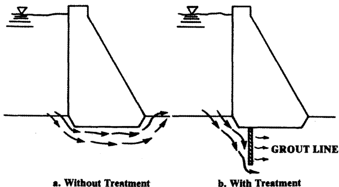
FIGURE 3.6-5 GROUTED CUTOFF
