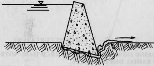
(b) Foundation starts to fail, allowing dam to be moved by the force of the water.
