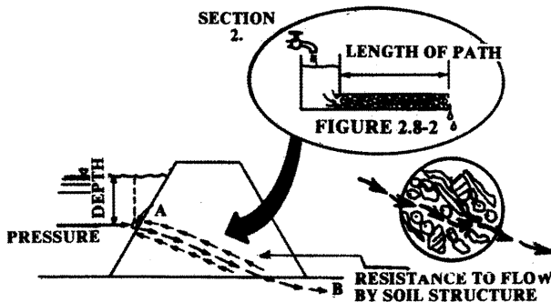
FIGURE 3.4-4 RESISTANCE TO FLOW
