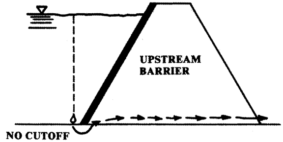
FIGURE 3.4-10 FLOW PATH IN COARSE MATERIAL WITHOUT CUTOFF
