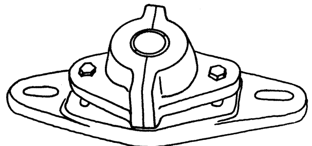
SPLIT CASE STEM GUIDE WITH SPLIT METALLIC BUSHING INSERT. BUSHING INSERTS ARE USUALLY BRONZE OR NON-METALLIC.
