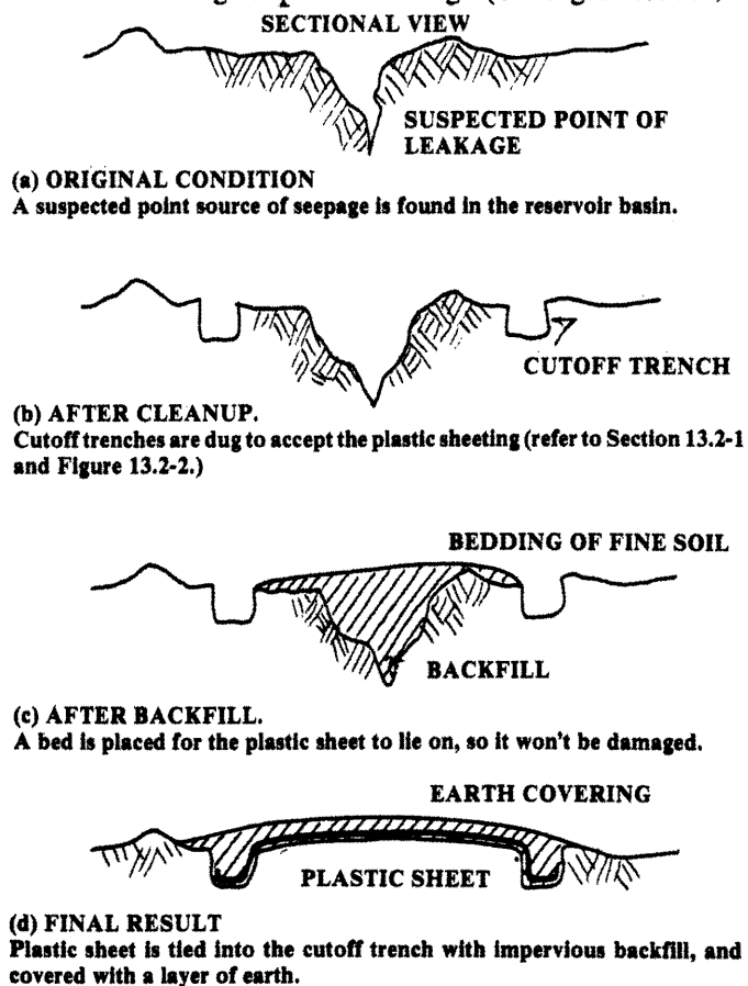
FIGURE 13.2-5 SEALING RESERVOIR BASINS AGAINST MINOR LEAKAGE BY USE OF PLASTIC SHEETING
