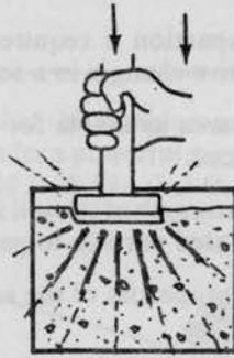
FIGURE 2.5-6 TRANSMISSION OF COMPACTION FORCE
