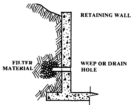
FIGURE 10.2 — WEEP HOLE
