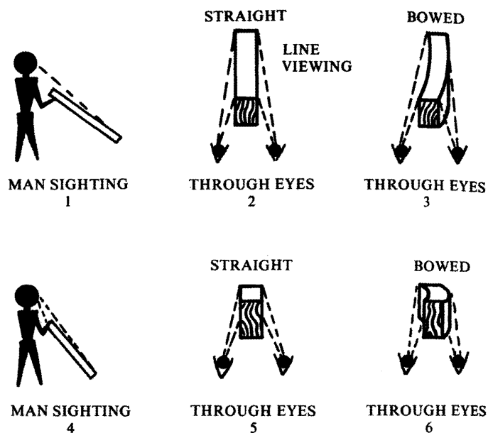
FIGURE 4.4-1 SIGHTING TECHNIQUE
