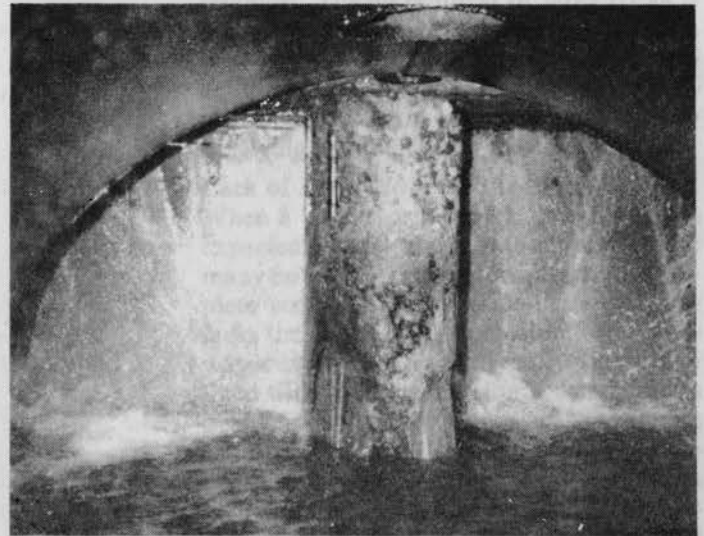
PHOTO 9.8-3 — SIDE BY SIDE SLIDE GATES Gate leakage and cavitation damage to bull nose pier. Note exposed reinforcing steel. Air vent pipe at top of photo.
