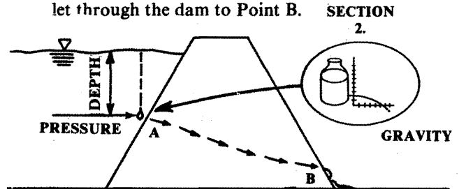
FIGURE 3.4-1 SEEPAGE PATH
