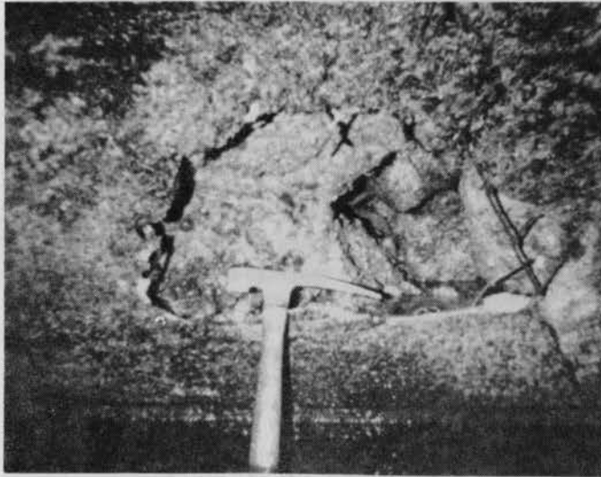
PHOTO 9.8-1 — OUTLET — INTERNAL EROSION Hole in cast-in-place concrete lining, caused by turbulence and erosion.
