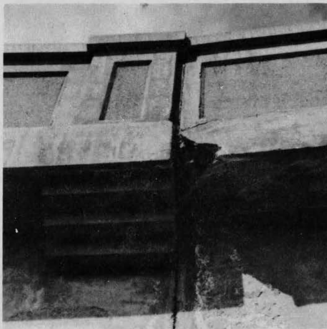
PHOTO 11.4-1 CRACK AT VERTICAL CONSTRUCTION JOINT. Note evidence of minor leakage and spalling adjacent to joint.
