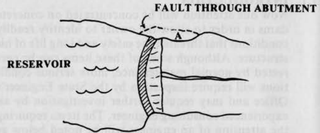
(A) CONCRETE ARCH DAM WITH A FAULT PLANE CUTTING THROUGH ONE ABUTMENT. Block "A" is unstable.
