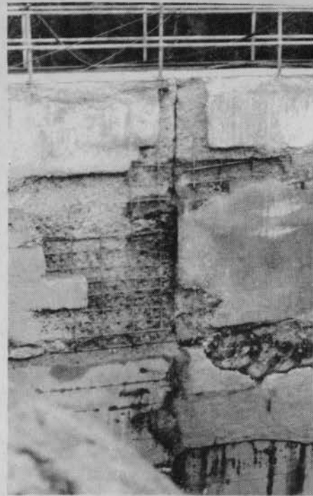
PHOTO 11.4-4 SEVERE SPALLING HAS EXPOSED REINFORCEMENT ON THE UPSTREAM FACE OF THIS DAM.
