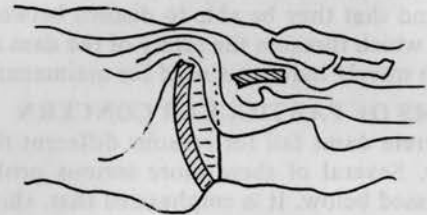
FIGURE 11.3 ABUTMENT FAILURE OF A CONCRETE ARCH DAM. (Drawings are in plan view.)
