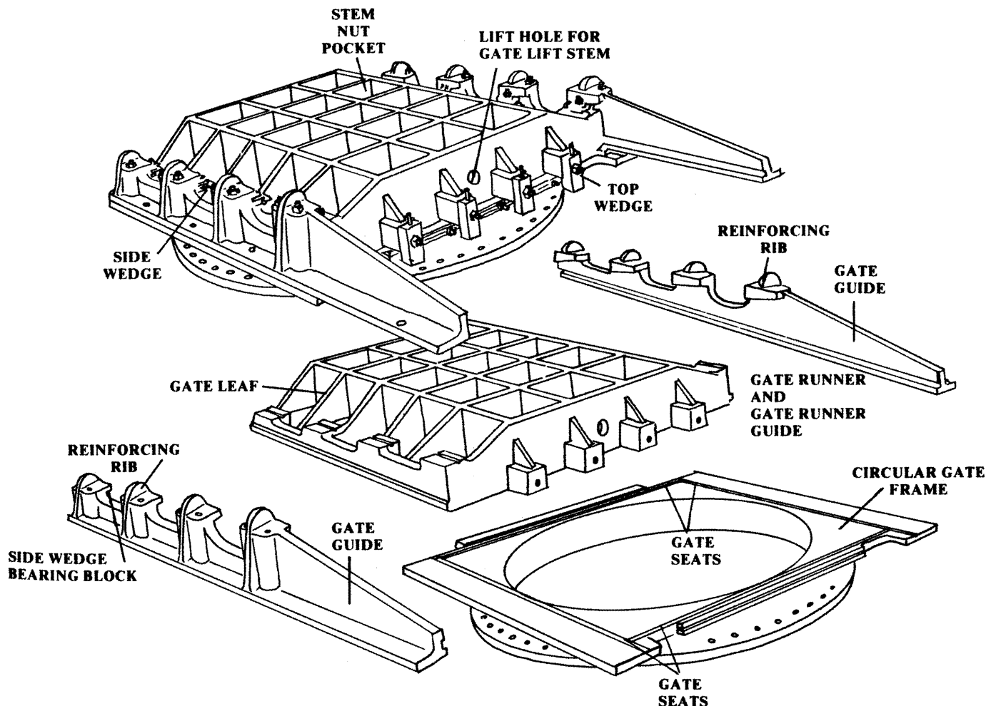
FIGURE 13.6-2 — BASIC COMPONENTS OF AN OUTLET GATE INSTALLATION
