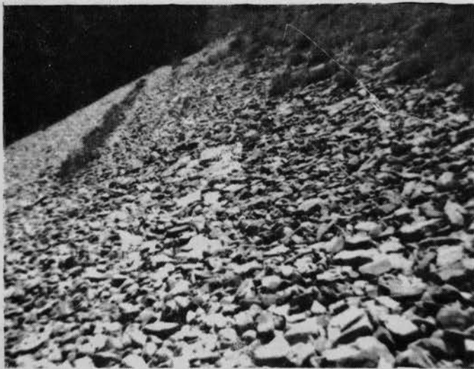
PHOTO 8.4-3 — EXAMPLE OF WELL-PLACED RIPRAP ON THE DOWNSTREAM SLOPE
