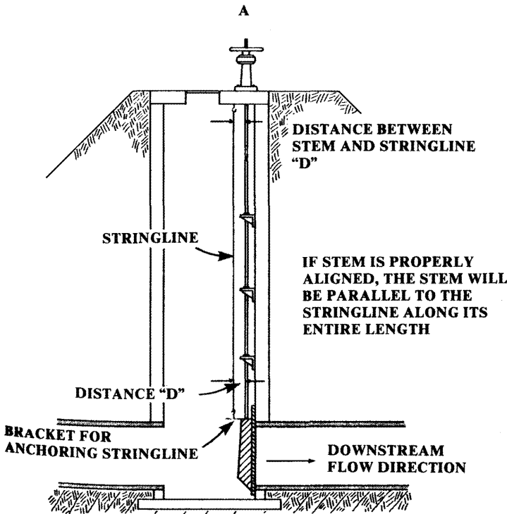
FIGURE 13.6-6.a — CHECKING STEM ALIGNMENT IN THE UPSTREAM/DOWNSTREAM DIRECTION
