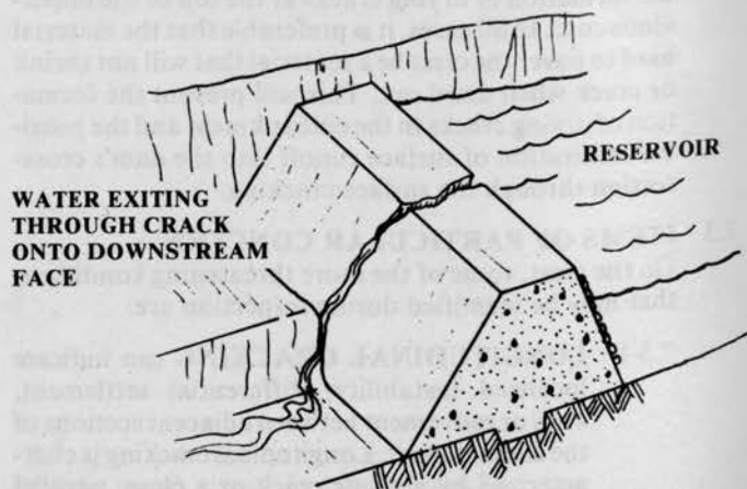
B) Progression of Transverse Crack to a Point Below the Waterline.
