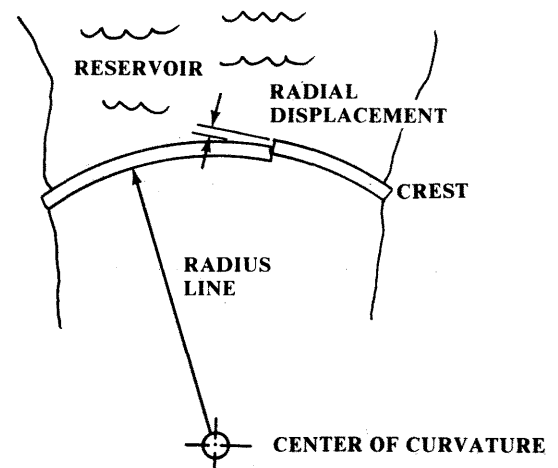
(B) VIEW LOOKING DOWN ON CONCRETE ARCH DAM. NOTE CRACK WITH RADIAL DISPLACEMENT.
