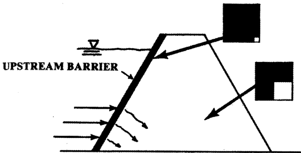
FIGURE 3.4-8 UPSTREAM BARRIER
