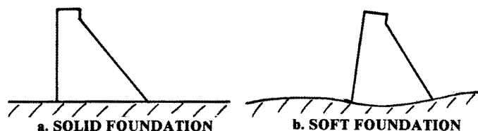
FIGURE 3.2-3 FOUNDATION CONDITIONS
