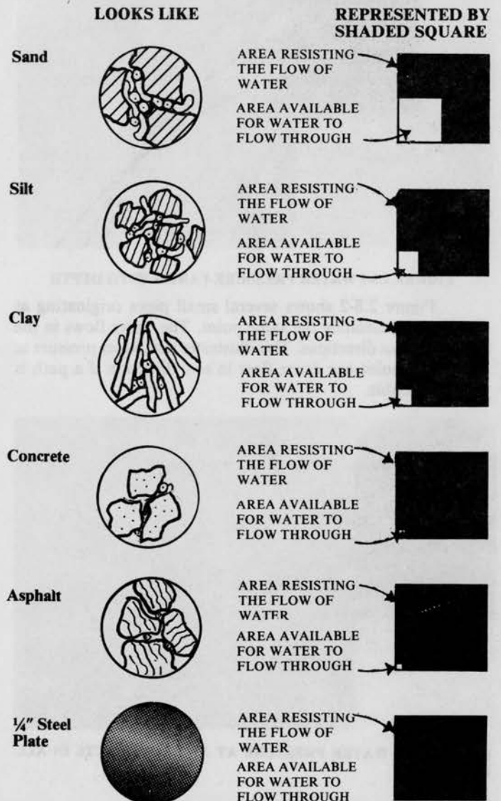
FIGURE 2.7-1 — COMPARISON OF AREA AVAILABLE FOR WATER TO FLOW THROUGH . (NOT TO SCALE)
