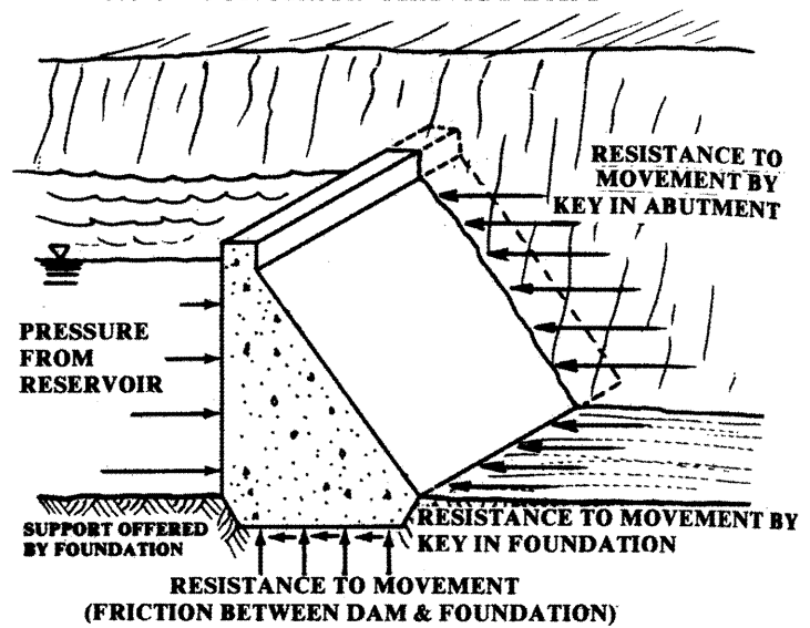
FIGURE 3.6-1 CONCRETE GRAVITY DAM
