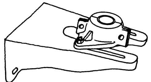
SPLIT CASE STEM GUIDE MOUNTED ON WALL BRACKET. THIS GUIDE HAS A SOLID METAL BUSHING INSERT.
