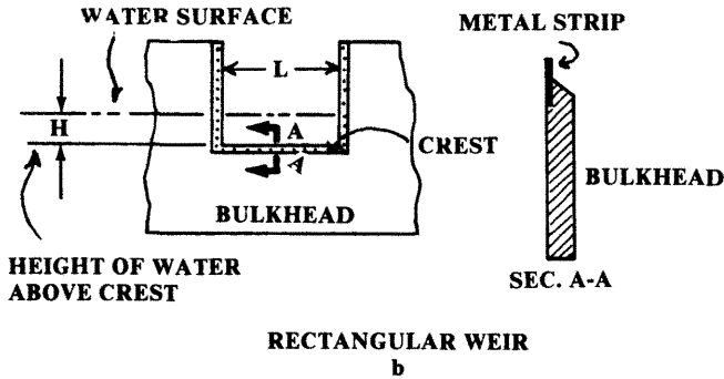
FIGURE 12.4-3 — STANDARD WEIRS
