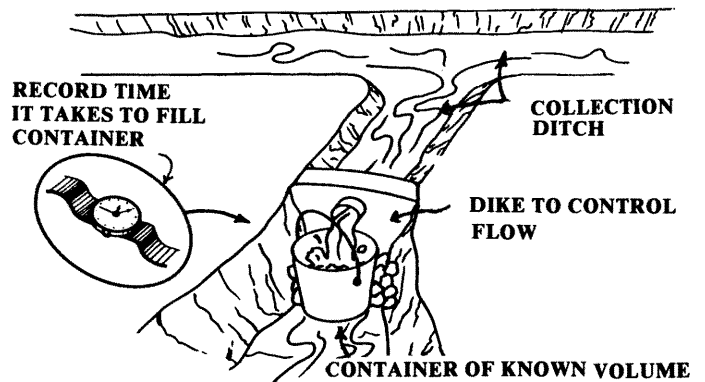
FIGURE 12.4-2 — BUCKET AND STOPWATCH METHOD
