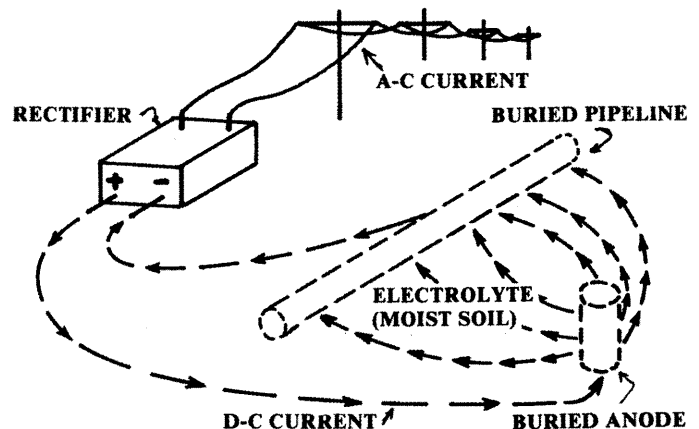
Field Installation of IMPRESSED-CURRENT (Rectifier-groundbeds) cathodic protection.
