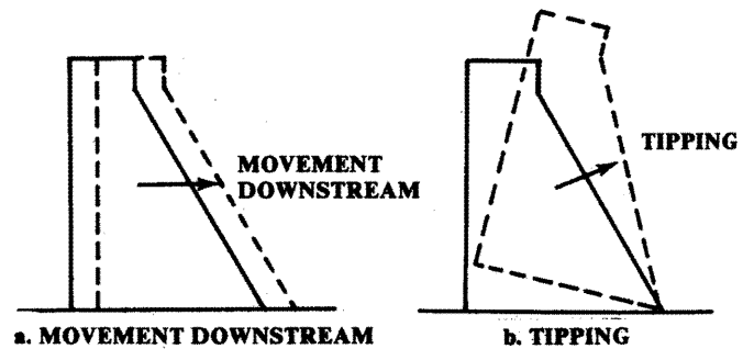
FIGURE 3.6-2 GRAVITY DAM MUST RESIST RESERVOIR LOADS
