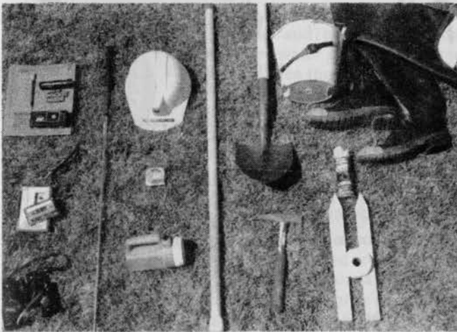
FIGURE 4.2-1 INSPECTION EQUIPMENT — Notebook, pencil, hand-level, camera, tape recorder and tape, binoculars, probe, hard hat, pocket tape, flashlight, bonker, shovel, rock hammer, bucket and stopwatch, bug spray, flagging tape and stakes, waterproof boots.
