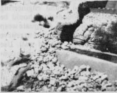
PHOTO 10.5-1 — FAILED SPILLWAY GABION WALL
