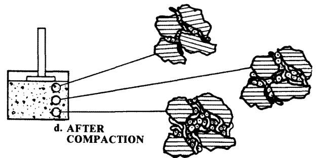
FIGURE 2.5-6 RESULT OF COMPACTION WITHOUT CONTROLLED LAYERS.
