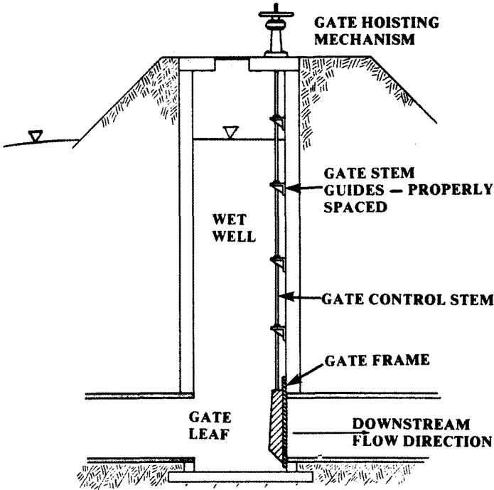
FIGURE 13.6-4 — WET WELL OUTLET INSTALLATION
