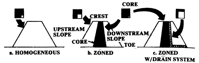
FIGURE 3.4-5 TYPICAL CROSS SECTIONS
