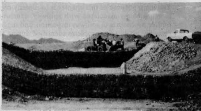
PHOTO 10.4-1 — GABION DROP STRUCTURE. A special type of rock protection against erosion.
