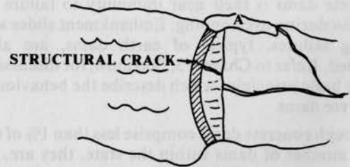
(B) BLOCK "A" MOVES DOWNSTREAM REDUCING SUPPORT FOR THE DAM. A structural crack develops, and seepage begins at weak abutment and through dam.
