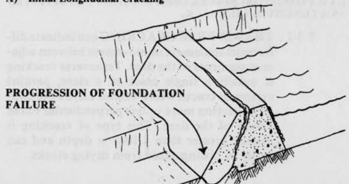
B) Progression of Longitudinal Cracking
