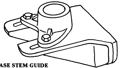
SOLID CASE STEM GUIDE MOUNTED ON WALL BRACKET
