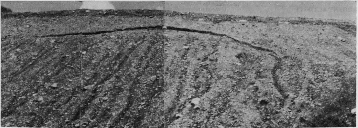
PHOTO 8.5-2 — TRANSVERSE CRACKING
