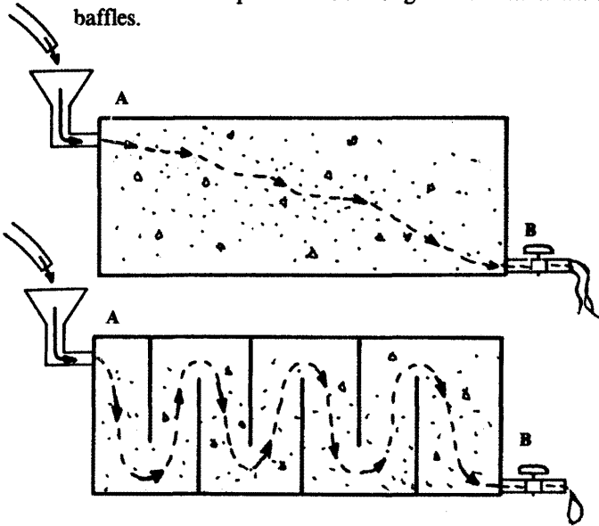
FIGURE 2.10-2 ANOTHER WAY TO INCREASE THE FLOW PATH Although the height of water above Point B is equal for both tanks the flow from the tank having the longer flow path will be much less.
