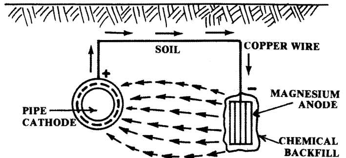
CATHODIC PROTECTION: GALVANIC ANODE (From: Joseph F. Bosich, CORROSION PREVENTION FOR PRACTICING ENGINEERS , Barnes & Noble, 1970)
