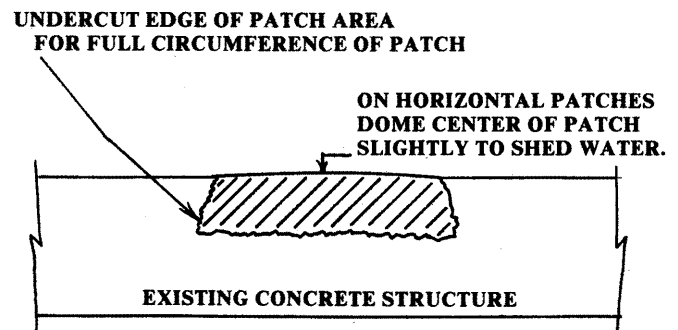
FIGURE 13.4-1 — CONCRETE PATCH
