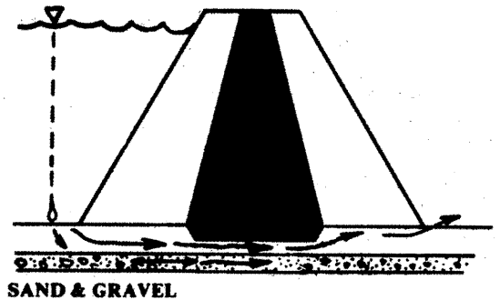
a. Cutoff Too Shallow
