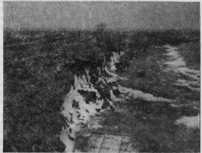
PHOTO 6.2 — EROSION OF UPSTREAM FACE DUE TO LACK OF PROTECTION AGAINST WAVE ACTION.
