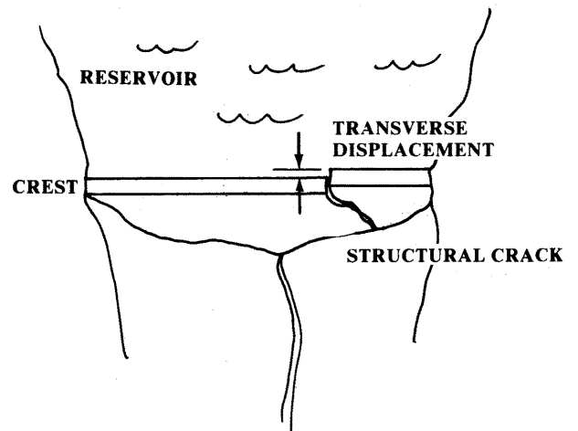
(C) VIEW LOOKING DOWN ON A CONCRETE GRAVITY DAM. NOTE IRREGULAR STRUCTURAL CRACK WITH TRANSVERSE DISPLACEMENT.
