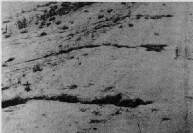
PHOTO 7.5-6 — RUNOFF GULLIES FORMING ON THE DOWNSTREAM SHOULDER OF THE CREST
