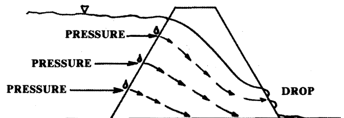
FIGURE 3.4-2 FLOW PATH
