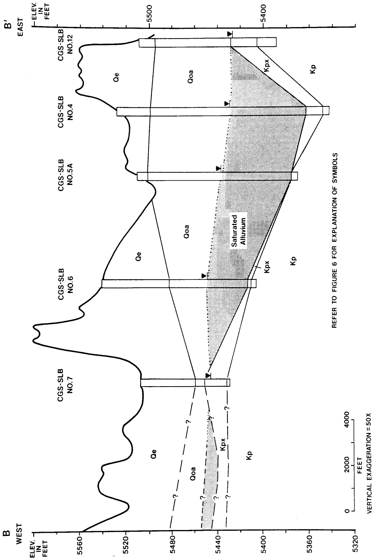
Figure 9. East-west cross section (B-B') in the southern part of the project area.
