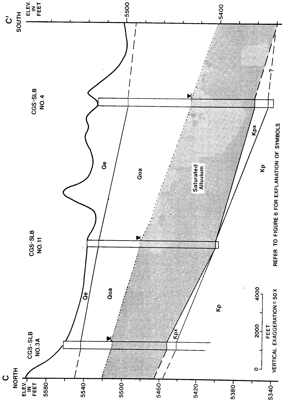
Figure 10. North-south cross section (C-C') along the center of the buried channel.
