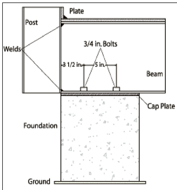
Figure 9. Option 2, beam extends a great distance on foundation and beam is bolted to foundation.
