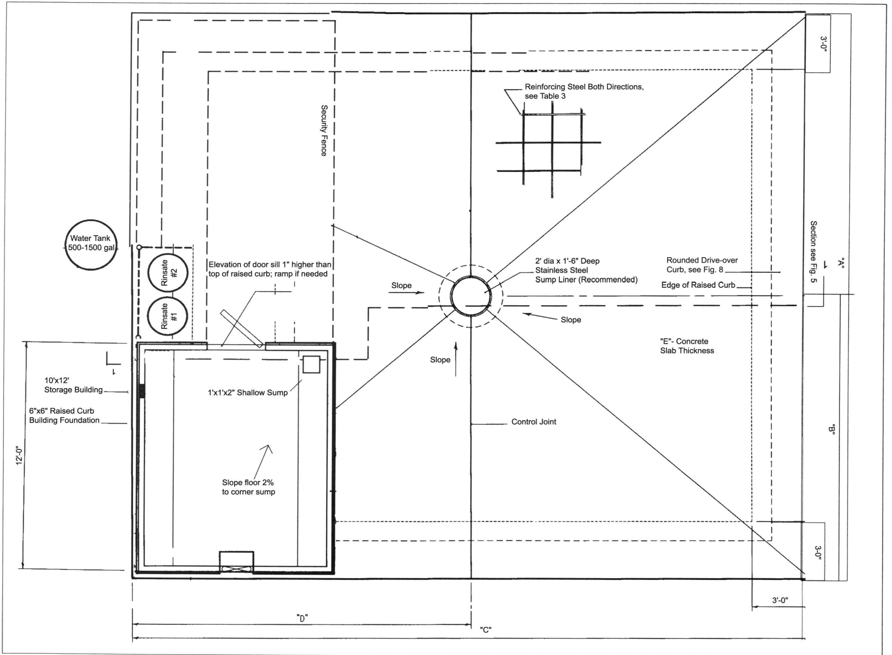
10 Figure 4. Plan view of single sump mixing/loading pad with pesticide storage. See Table 1 for dimensions.
