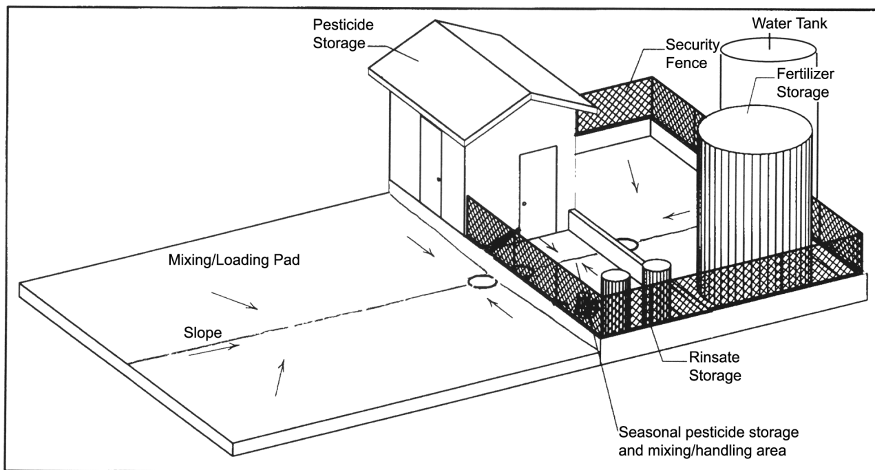
Figure 10. Secondary containment for fertilizer and pesticide storage with mix/load pad.
