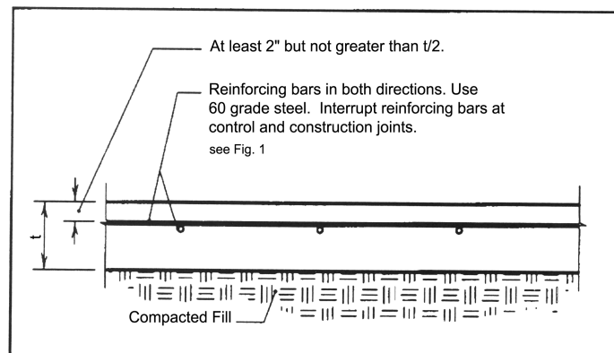
Figure 9. Mixing/loading pad structural design. See Table 3 for thickness and steel reinforcement requirements.
