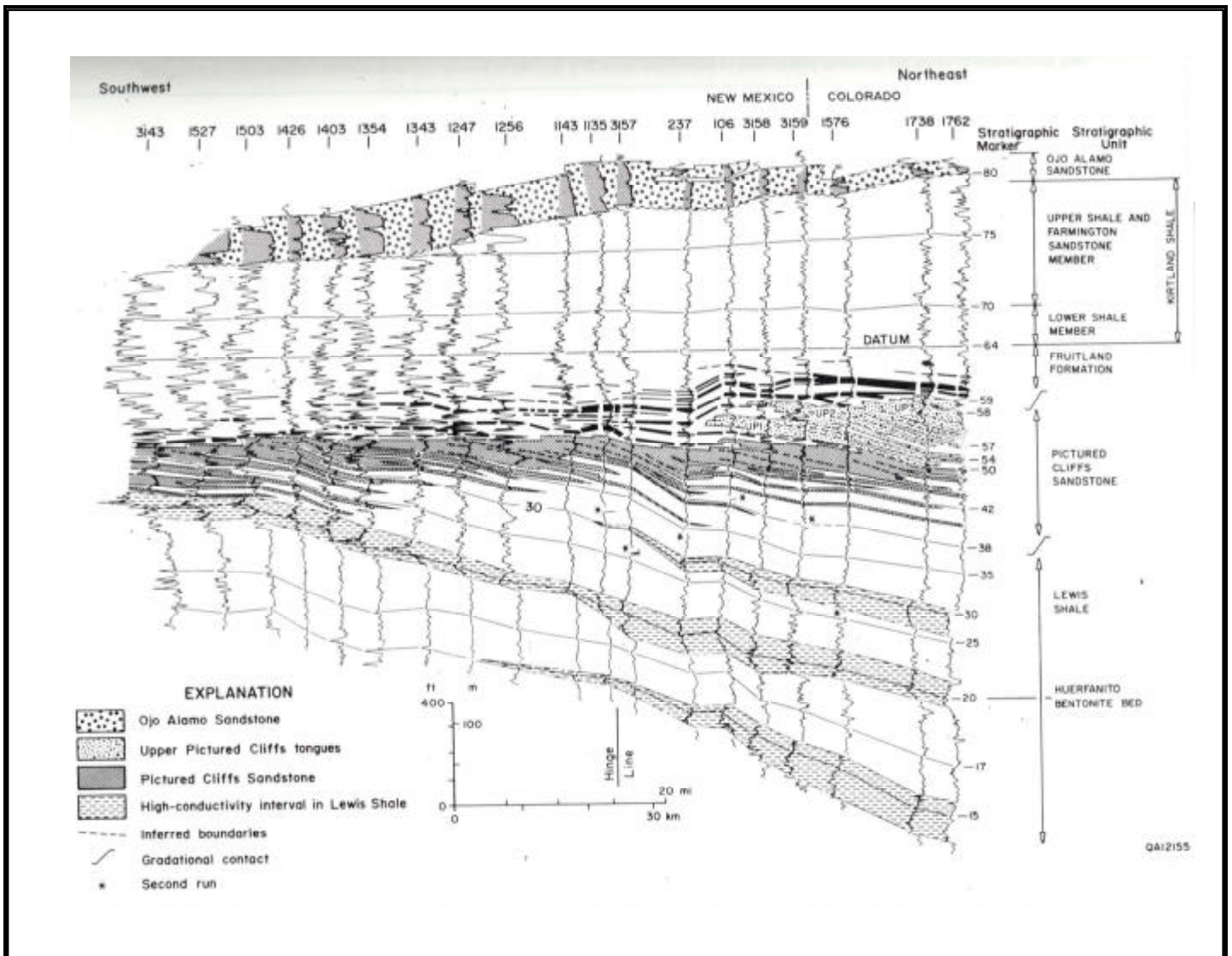
Figure 3.4. Fruitland-Pictured Cliffs Stratigraphic Cross Section
