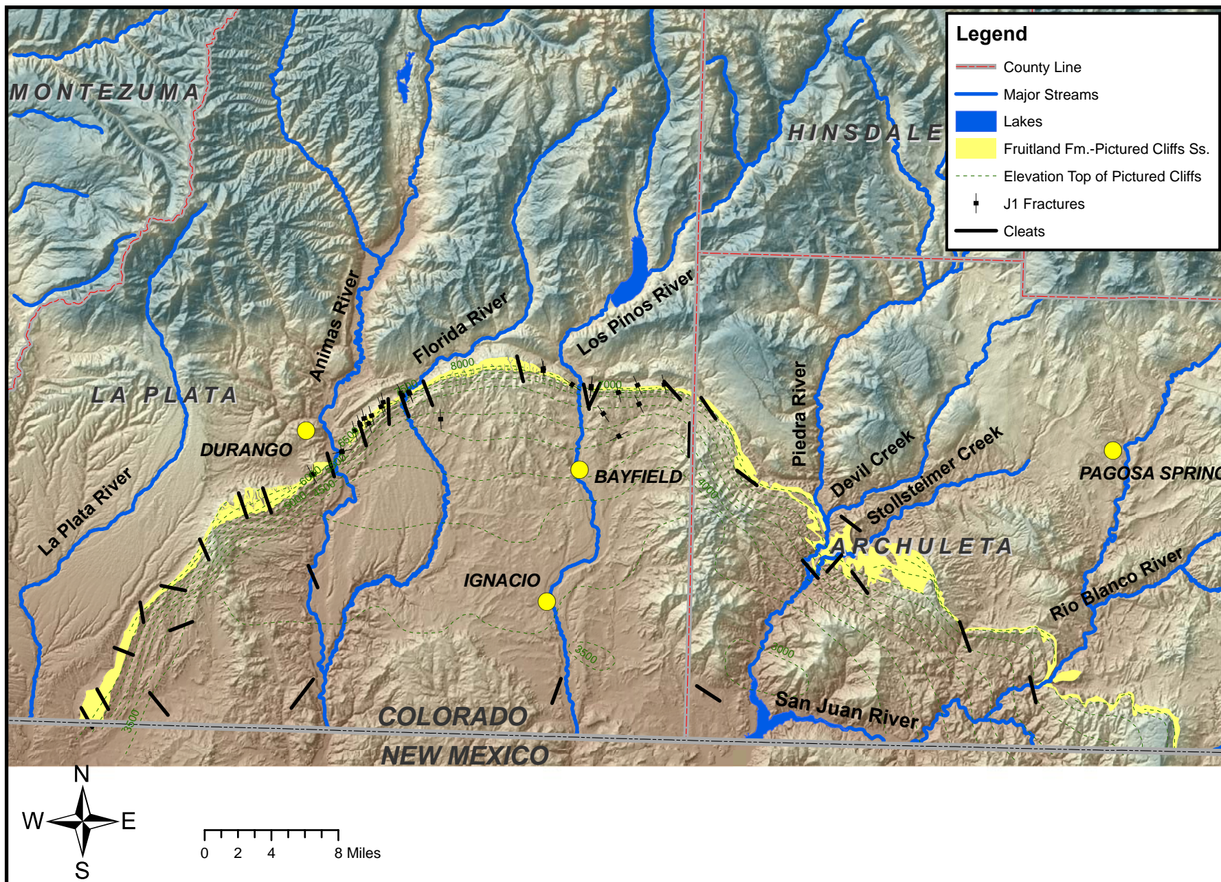
Figure 3.6. J1 Fracture and Coalbed Face Cleat Orientation, Northern San Juan Basin
