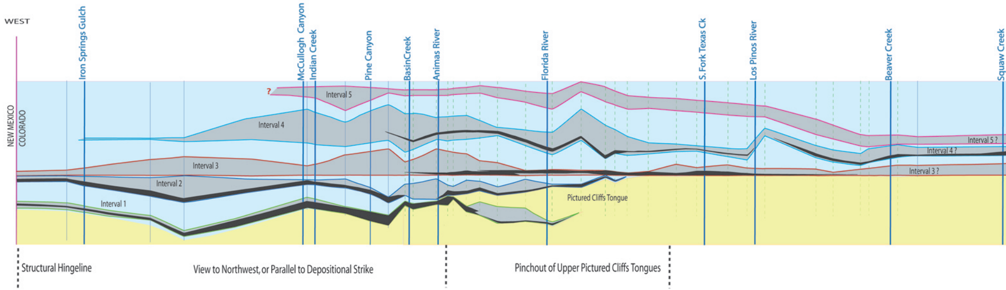
Figure 3.8. □ Fruitland Formation Coal Intervals Along the Outcrop, Northern San Juan Basin, Colorado
