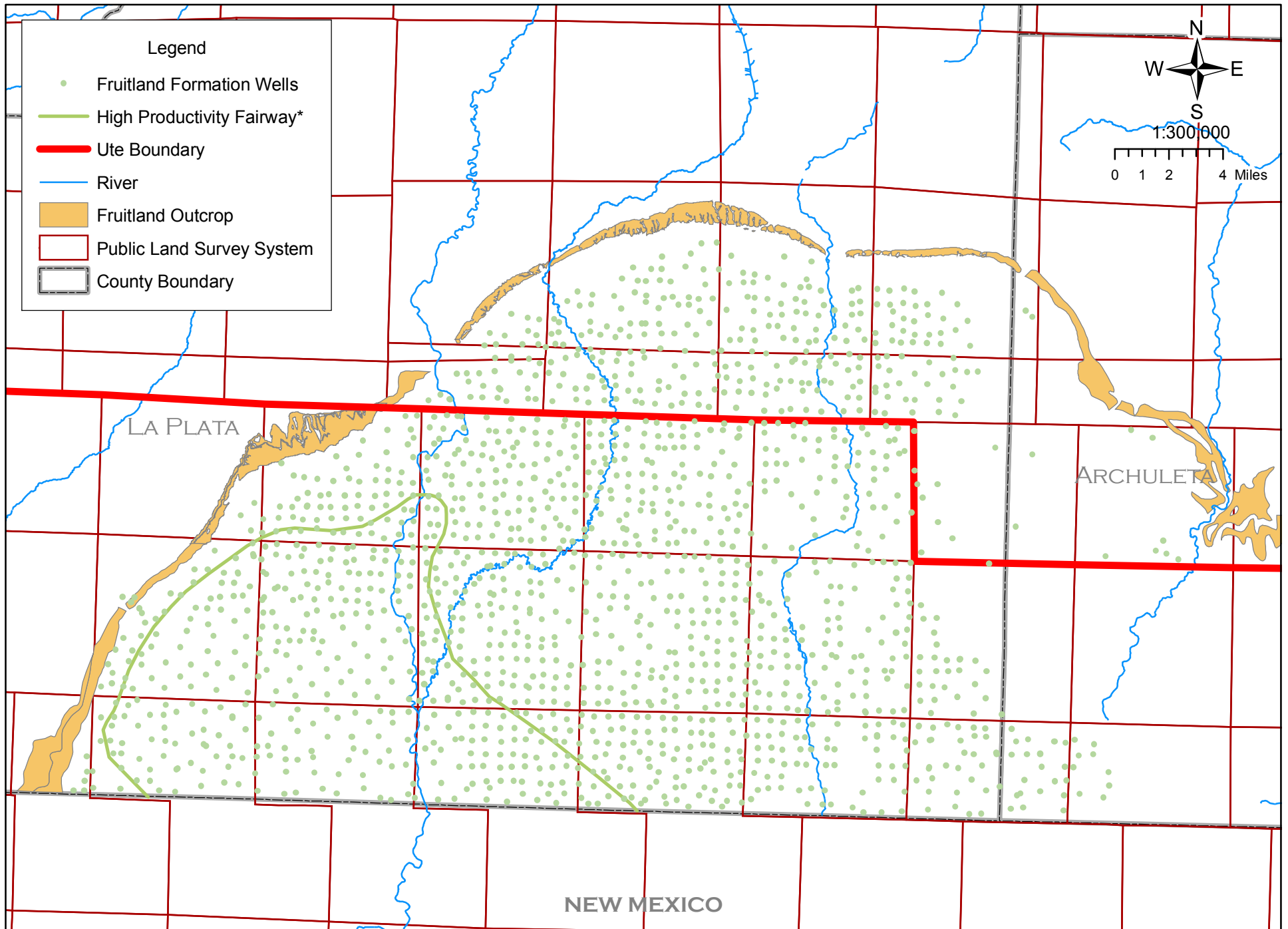
Figure 4.1. High Productivity Fairway (*Based on Tyler, 1997; Figure 7)
