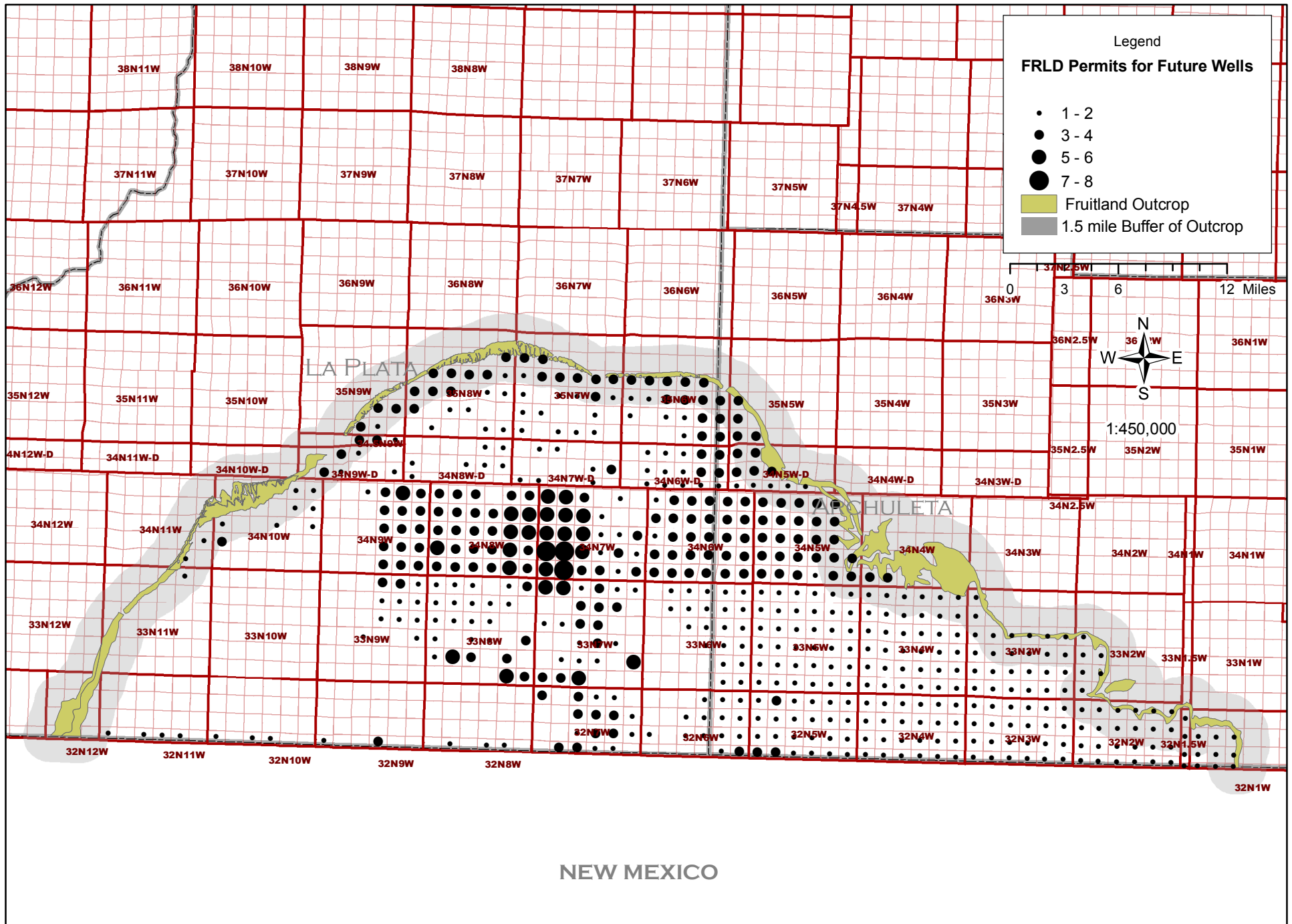
Figure 6.2. Potential Future Fruitland CBM Well Locations Used in Glover Analysis
