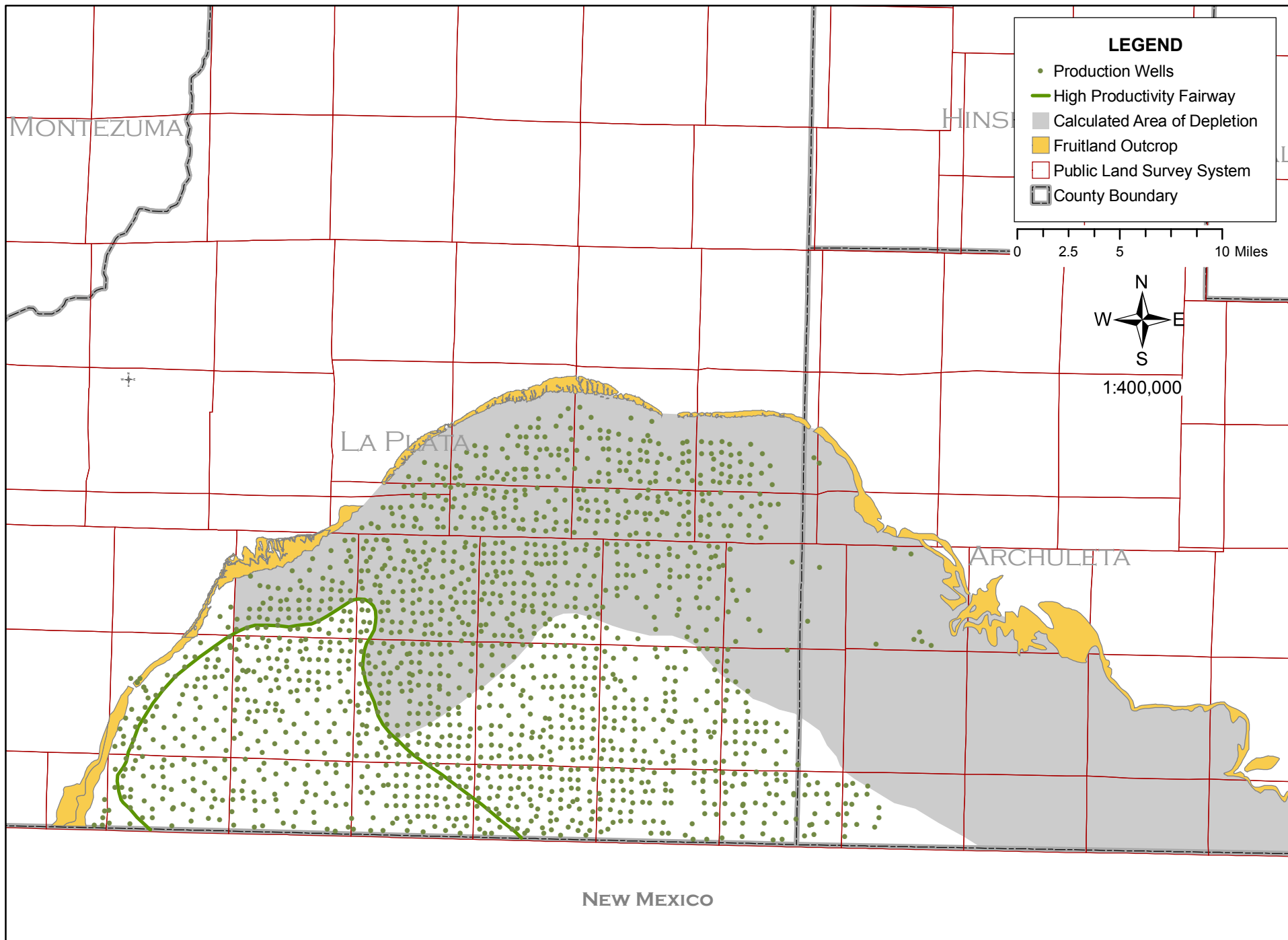
Figure 6.1. Area with Calculated Depletions exceeding 0.1% in 100 years
