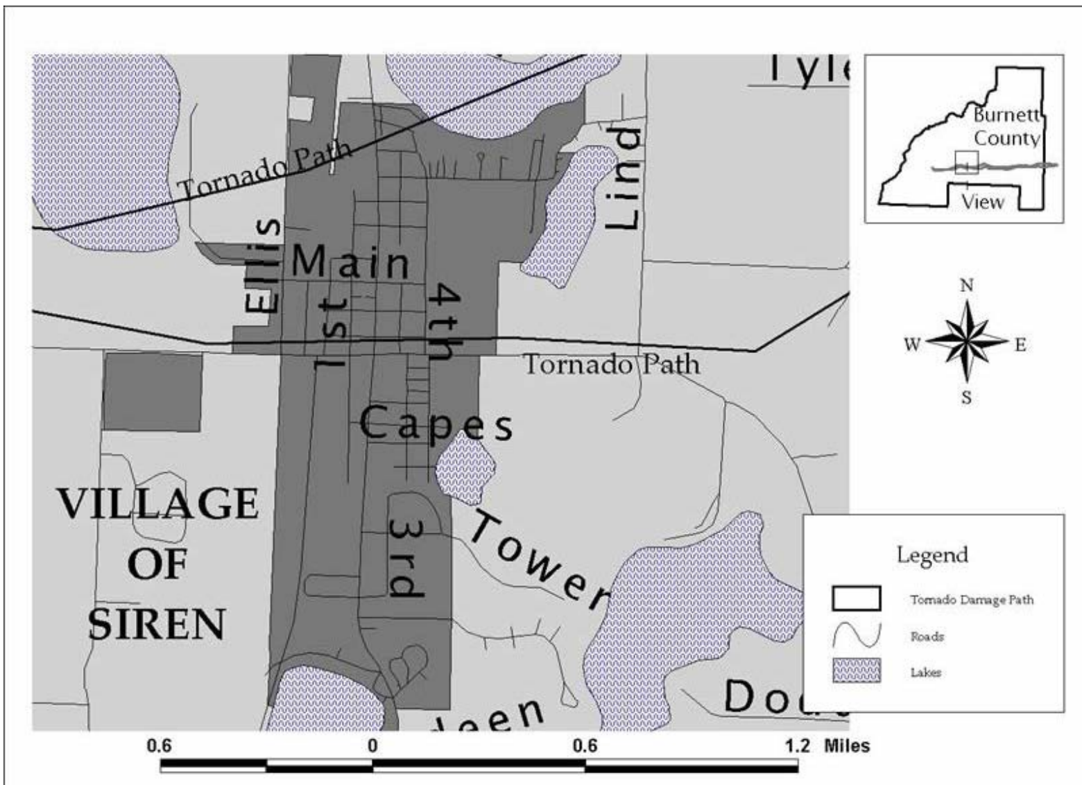
Figure 2. Tornado damage path through the Village of Siren, Wisconsin.
