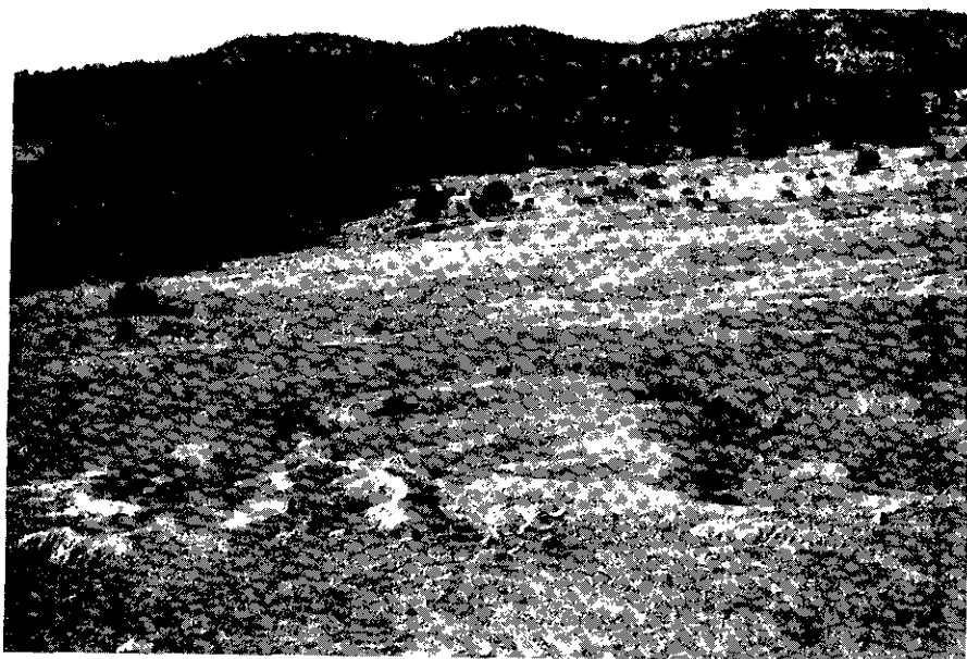
Rangeland erosion due to overgrazing
