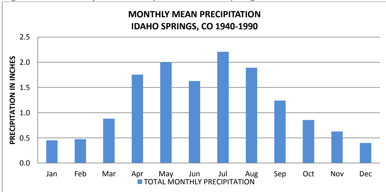
Figure 4. Monthly Mean Precipitation, Idaho Springs
