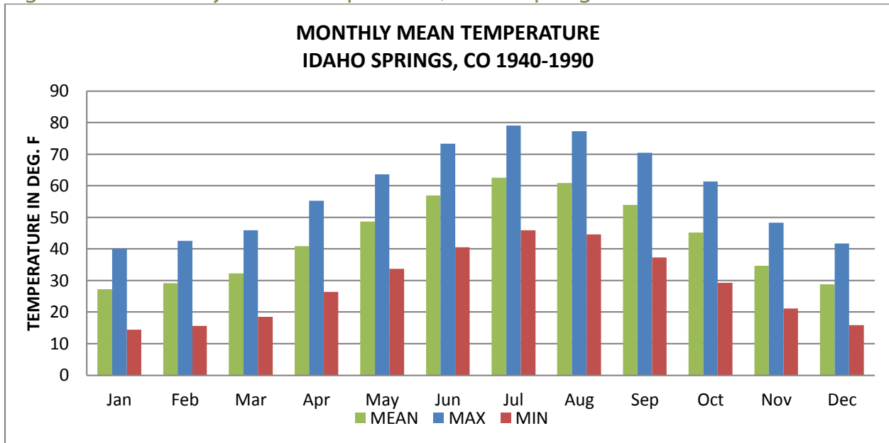
Figure 3. Monthly Mean Temperature, Idaho Springs
