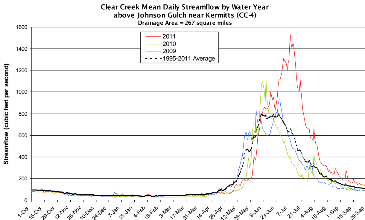
Figure 5. Clear Creek Mean Daily Discharge by Water Year
