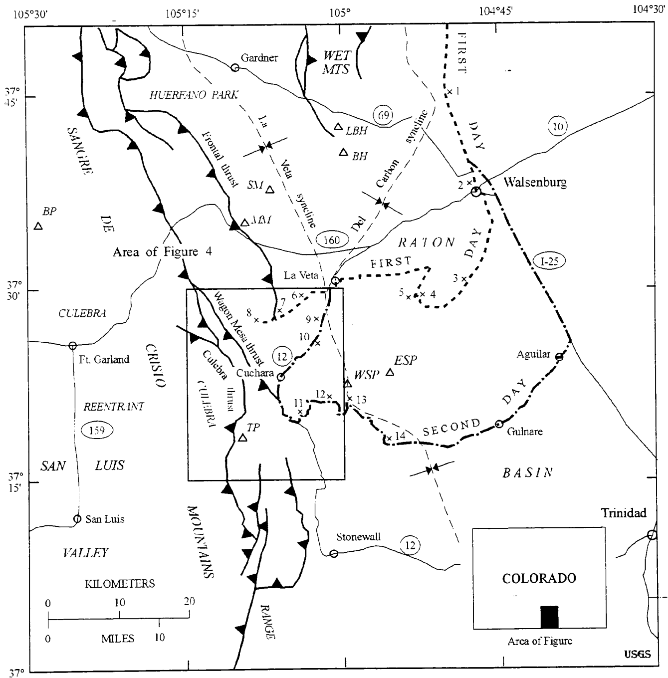
Figure 1.—Field trip route and structural setting of the Raton basin in southern Colorado (modified from Johnson, 1969). Geographic features on map: BP, Blanca Peak, BH, Black Hills; ESP, East Spanish Peak; LBH, Little Black Hills, MM, Mt. Mestas (Baldy); SM, Silver (Dike) Mountain; TP, Trinchera Peak; and WSP, West Spanish Peak.
