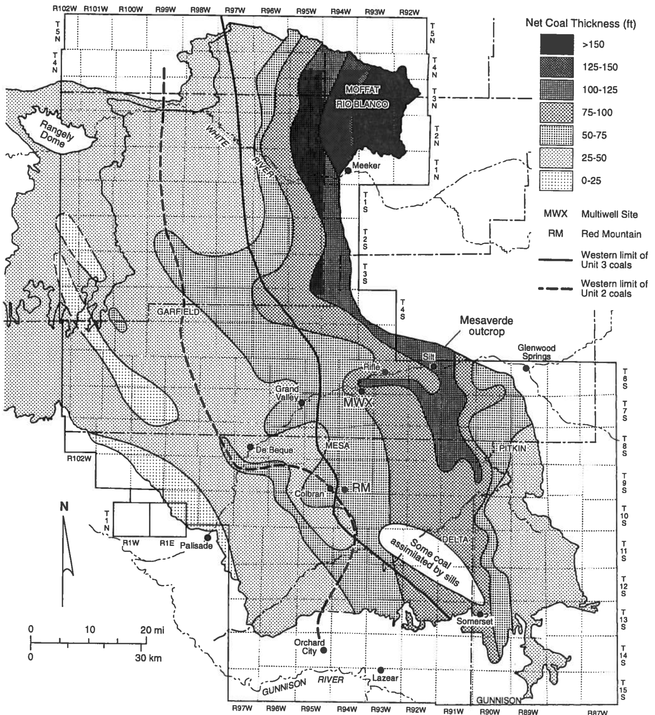
Figure 14. Net coal thickness map of genetic units 1 through 3, Williams Fork Formation. Northerly oriented net coal thickness trends in the eastern Piceance Basin occur above thick, north-south-oriented progradational shoreline (strandplain/delta plain) systems.
