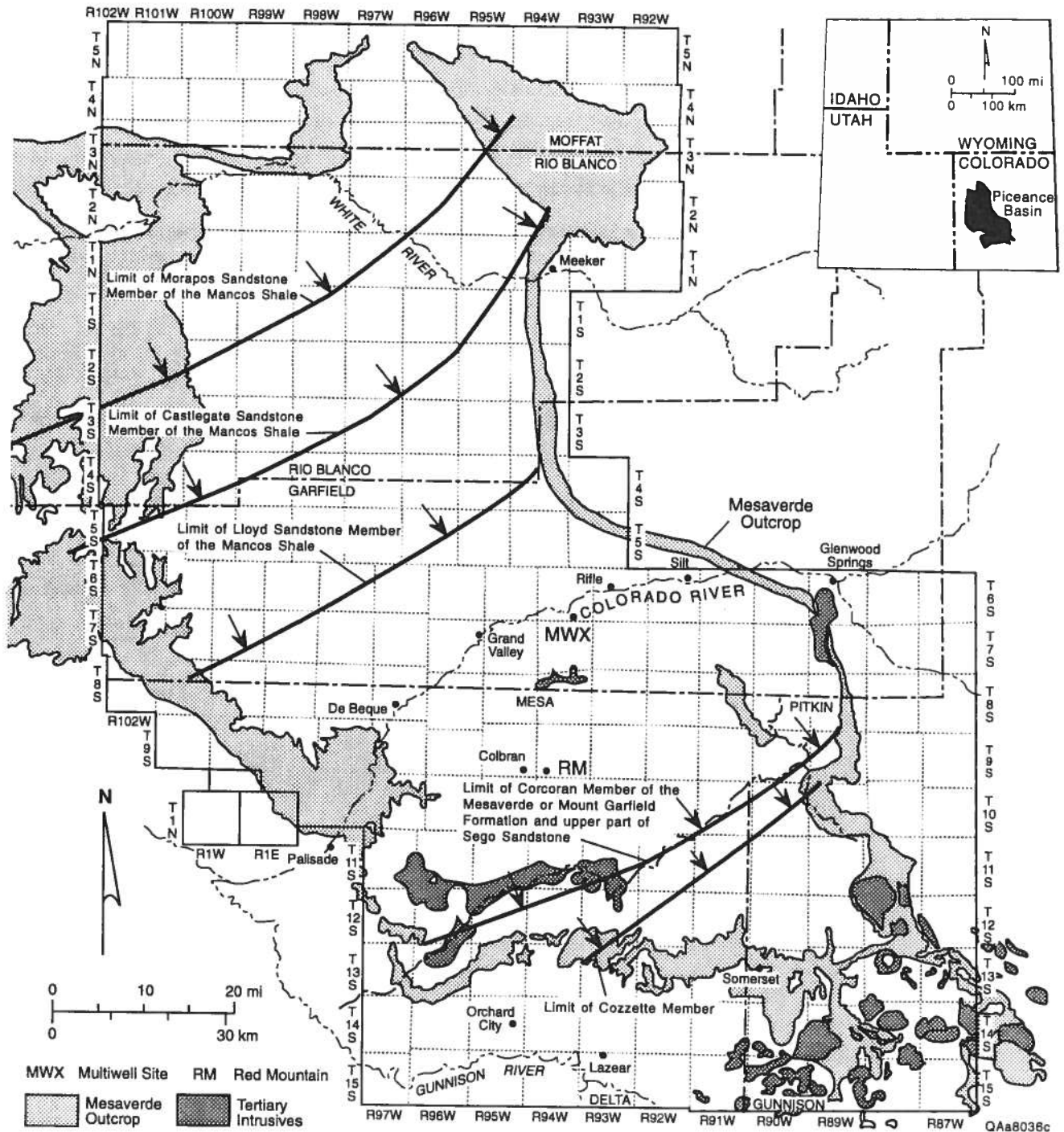
Figure 3. Regressive limits of the sandstone members of the Mancos Tongue and Iles Formation, Mesaverde Group. Limits of the Sege sandstone cannot be determined with certainty. Seaward limit of the Rollins-Trout Creek progradational sequence is beyond the southeastern corner of the Piceance Basin and the mapped area. Arrows indicate direction of regression. Modified from Zapp and Cobban (1960), Warner (1964), Gill and Cobban (1969), Gill and Hail (1975), and Johnson (1989).
