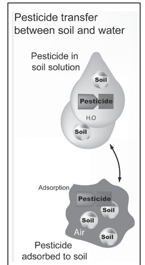
Figure 3. Pesticides will exist in the soil water solution, in soil air, or adsorbed onto soil particles.
