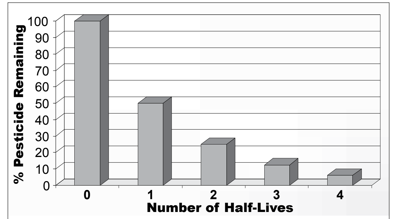
Figure 6. Half-life chart depicting conceptual pesticide degradation.
