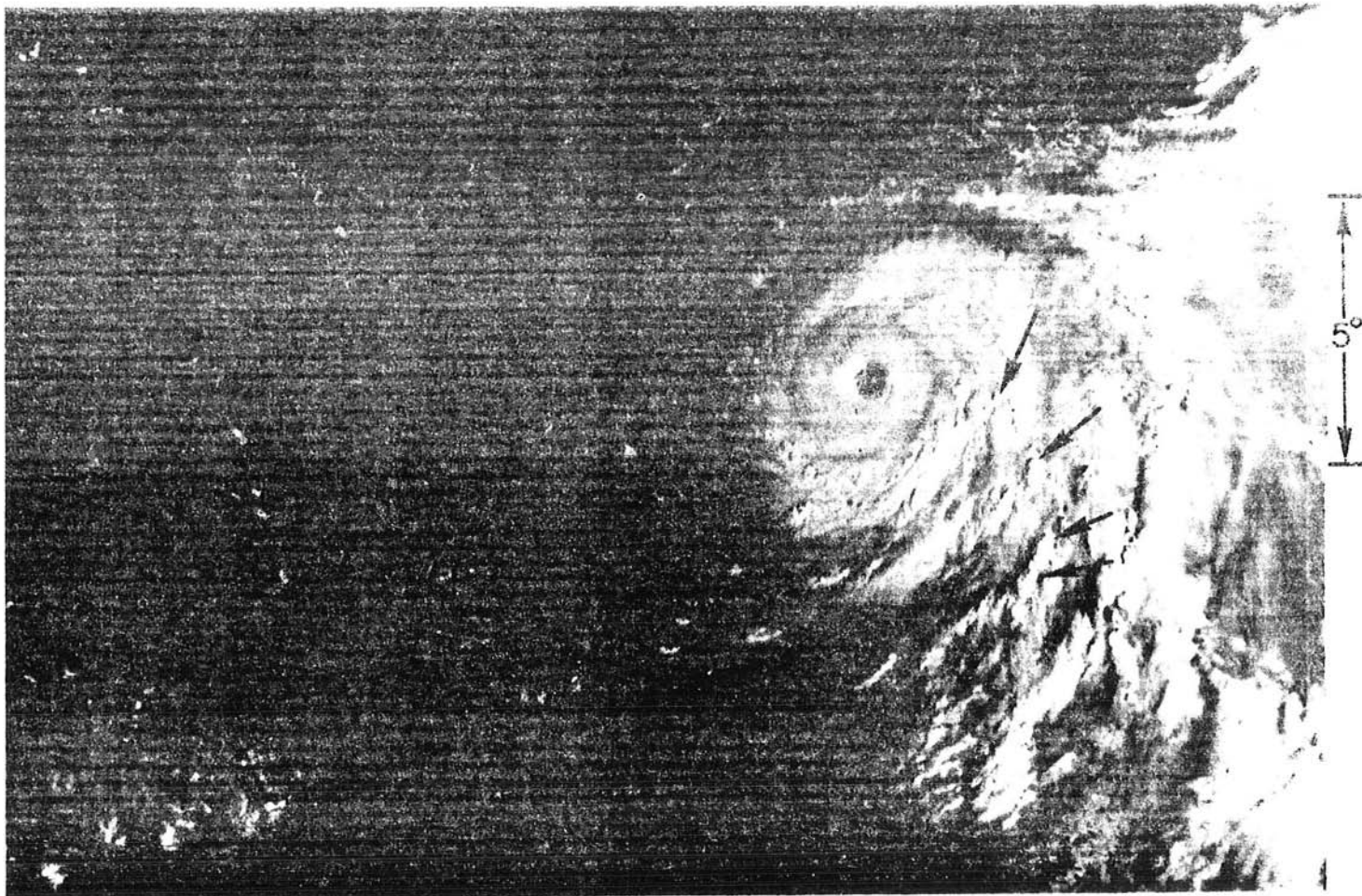
Fig. 24. Four typhoon cases with individual b asic c onvective e lements (BCE's) indicated by arrows. 1 in = 380 km. (a) Typhoon Wendy (Stage IV), 7 September 1971, 2107Z; (b) Same as (a) except for 8 September 1971, 2040Z; (c) Typhoon Pamela (Stage IV), 7 November 1972, 0012Z; (d) Same as (c) except for 7 November 1972, 0404Z.
