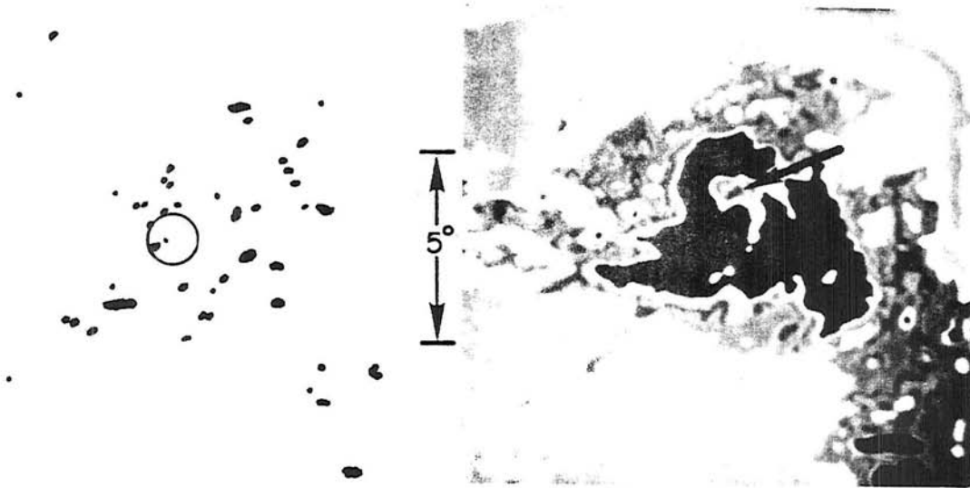
Fig. 10. Meso-convective elements of a developing cluster (Stage I) obtained from the tracing data set B. Storm's circulation center is within the circle. 1" = 484 km.
