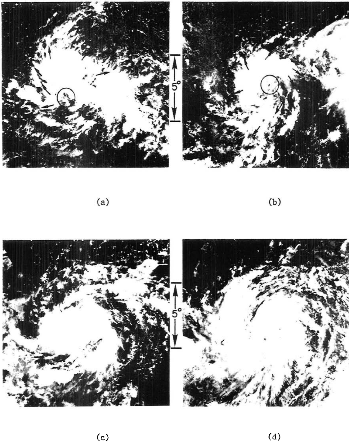
Fig. 20. An example of a storm (Typhoon Ora) which depicts the observed statistical trend of an average storm's life cycle, 1 in = 484 km. (a) Developing cluster (Stage I), 19 June 1972, 0228Z; (b) Tropical depression (Stage II), 22 June 1972, 0327Z; (c) Tropical storm (Stage III), 23 June 1972, 0312Z; (d) Typhoon (Stage IV), 23 June 1972, 2356Z. Circles in first two pictures show where low-level circulation center is located.
