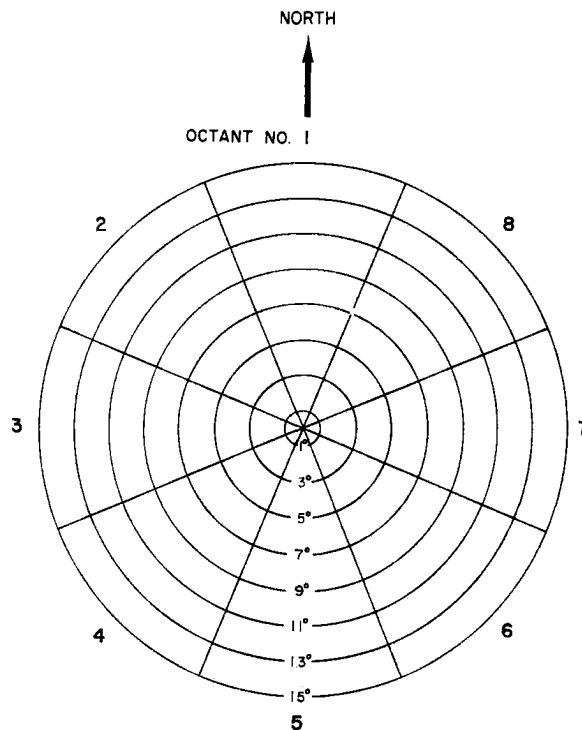
Fig. 17. Compositing grid used by Zehr (1976) and Frank (1976) with rawinsonde data sets.
