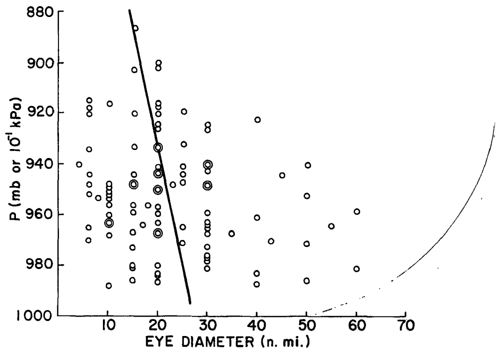
Fig. 19. Variation of eye diameter with central pressure. The best fit line is indicated by the heavy line.
