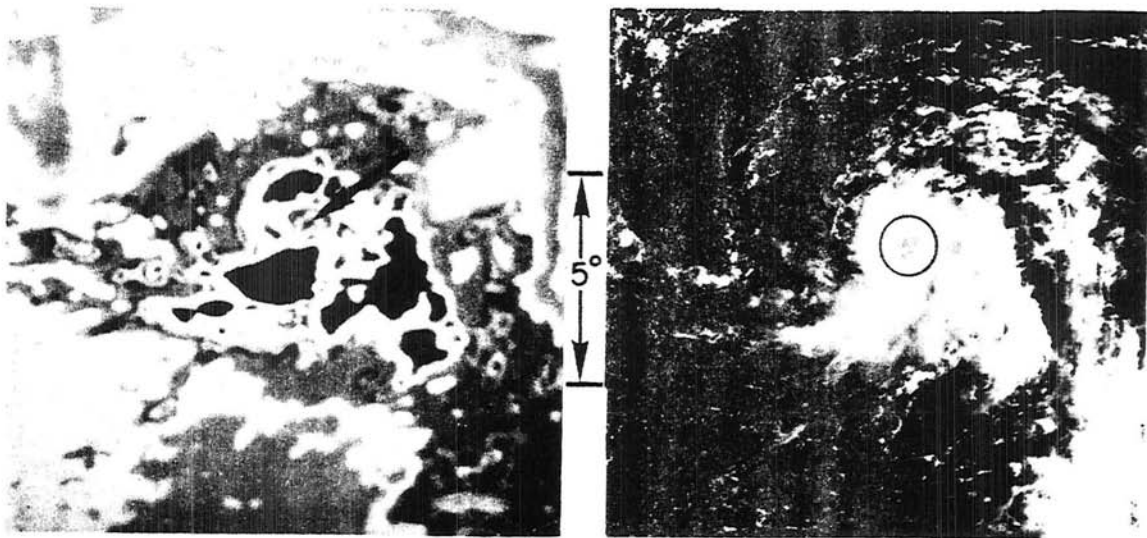
Fig. 12. Coldest shade (darkest shade) of cirrus ( T < 210K ) obtained from the infrared data set C for the cluster in Fig. 10. Arrow points to storm's circulation center. 1" = 484 km.
