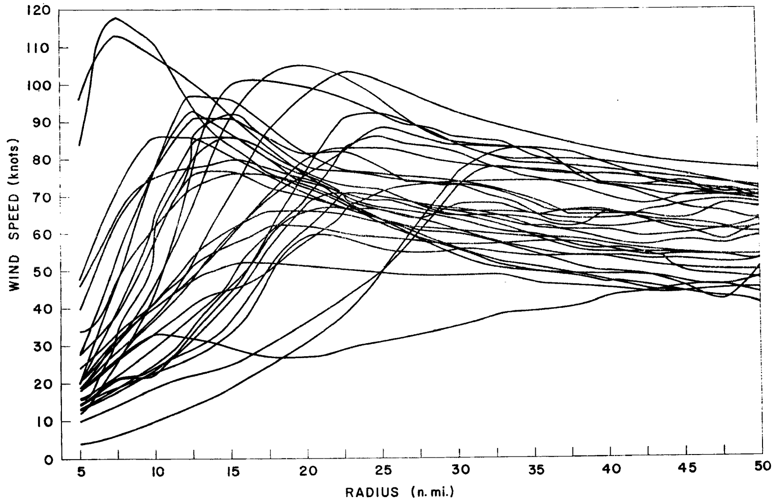
Fig. 7. Examples of observed tangential wind profiles (from Shea and Gray, 1973).
