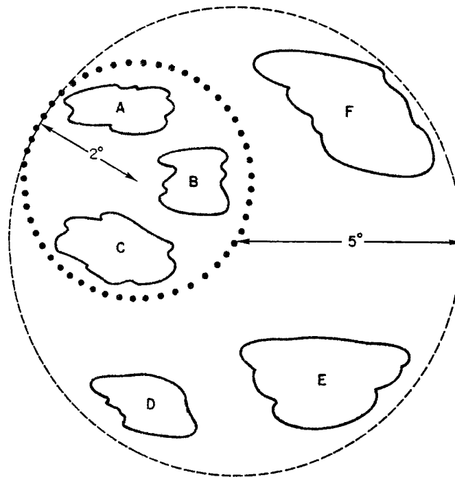
Fig. 18. Illustration of cluster definition. With poor resolution and contrast convective elements A, B, and C appear to merge and form a 4^{\circ} cluster. With improved resolution and contrast convective elements A-F are separable and form a 10^{\circ} cluster.
