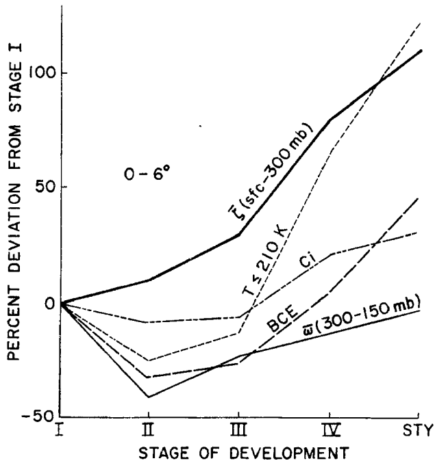
Fig. 58. Same as Fig. 56 except for r = 0-6^{\circ} .
