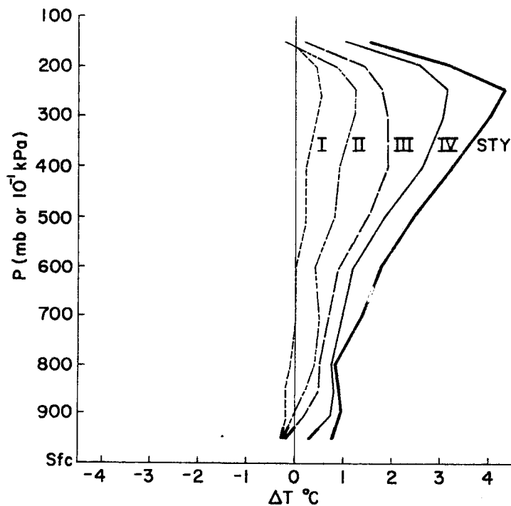
Fig. 51. Temperature anomaly profiles for five storm stages I, II, III, IV, and STY. \Delta T = \bar{T}(0-3^{\circ}) - \bar{T}(3-7^{\circ}) for stages I, II, III. \Delta T = (0-3^{\circ}) - 8^{\circ} for stages IV and STY.
