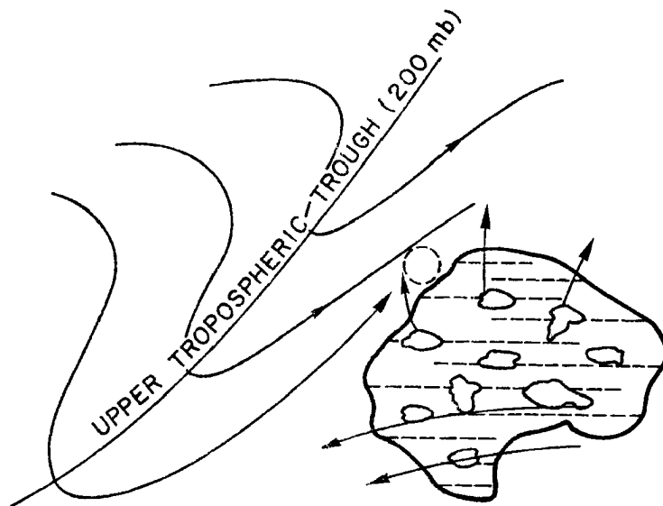
Fig. 32. Same as Fig. 31 except dynamically forced subsidence in an exposed clear region surrounding the cluster. Dashed circle represents area of maximum convergence between outflow from convective elements and southwesterly flow from upper level trough.
