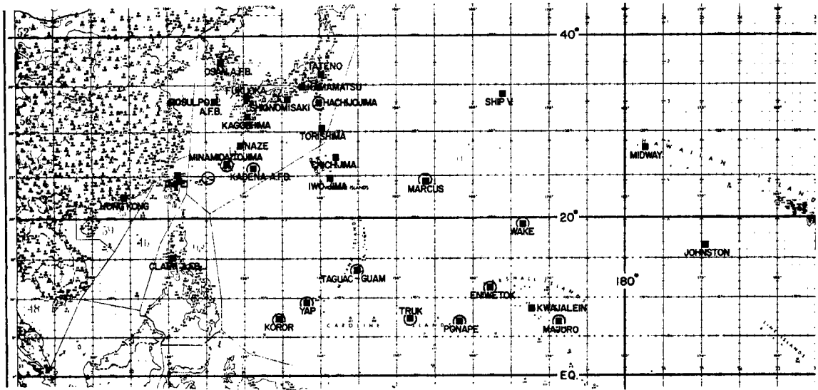
Fig. 16. Data network used in rawinsonde composites.
