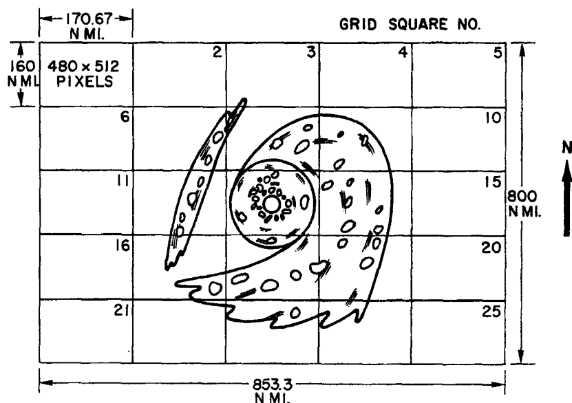
Fig. 14. Overlay grid centered on storm's circulation center and oriented north-south used to create visual and infrared data sets.
