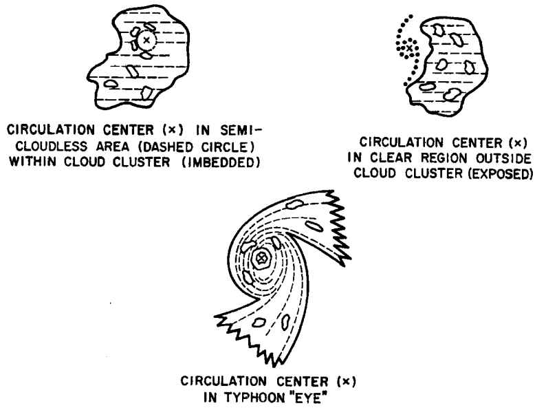
Fig. 8. Illustration of the three basic circulation center types associated with tropical cyclones.
