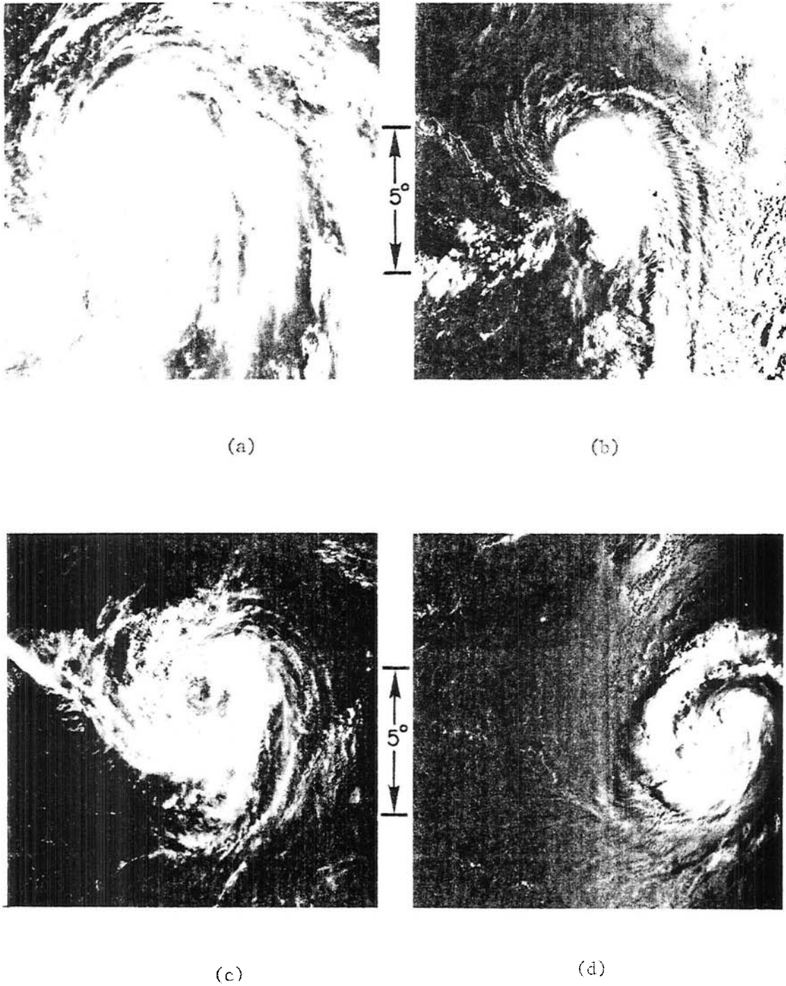
Fig. 42. Variability in cloudiness among typhoons (Stage IV), 1 in = 484 km. (a) Typhoon (Stage IV of Carmen), 16 October 1974, 0013Z; (b) Same as (a) except for Mary, 18 July 1971, 2041Z; (c) Same as (a) except for Alice, 7 August 1972, 0232Z; (d) Same as (a) except for Trix, 21 August 1971, 2206Z.
