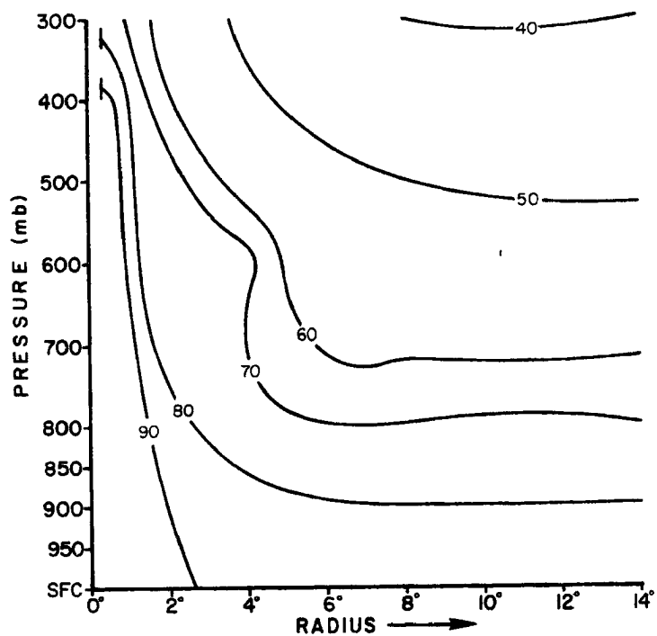
Fig. 55. Relative humidities of the typhoon stage at 1200Z (from Frank, 1976).
