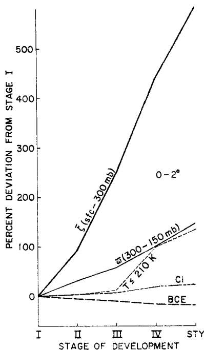
Fig. 56. Mean relative vorticity from the surface to 300 mb, mean vertical motion from 300 to 150 mb, percent area covered by basic convective elements (BCE), percent area covered by all cirrus (Ci), and percent area covered by the coldest cirrus ( T < 210 K) each expressed as a percent deviation from the corresponding developing cluster (Stage I) values. For r = 0-2^{\circ} .
