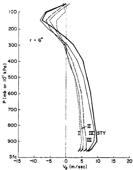
Fig. 50. Same as Fig. 48 except for r = 6^\circ .
