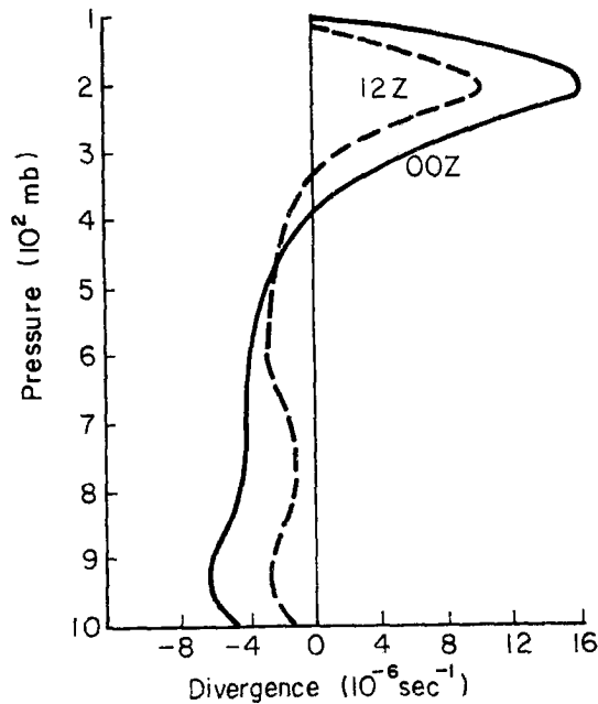
Fig. 59. Cloud cluster divergence (from Gray and Jacobson (1977)).
