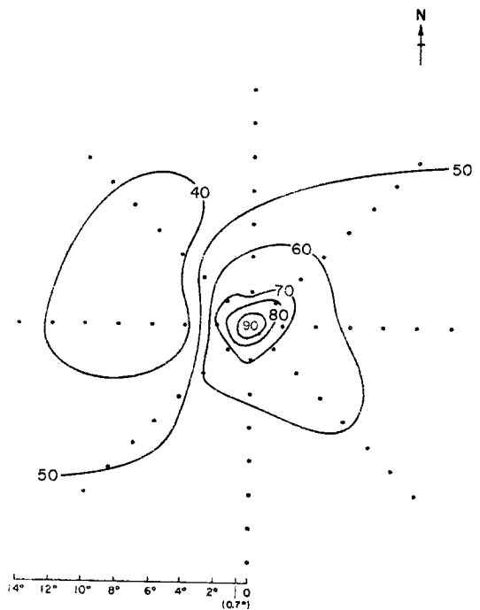
Fig. 54. Plan view of relative humidity at 500 mb for typhoon stage (from Frank, 1976).
