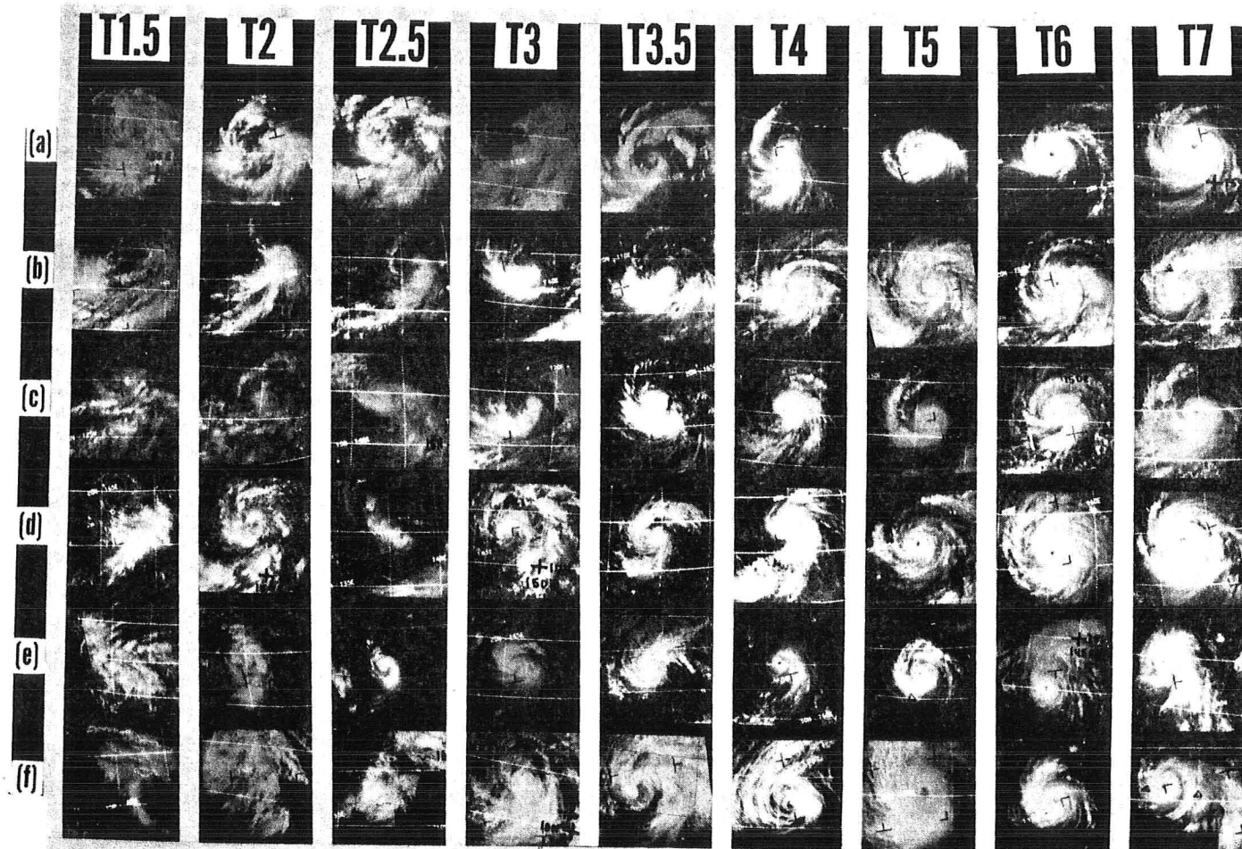
Fig. 3. Examples of preliminary T-number patterns (provided by V. Dvorak, 1975).
