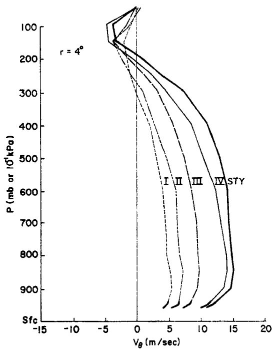
Fig. 49. Same as Fig. 48 except for r = 4^\circ .
