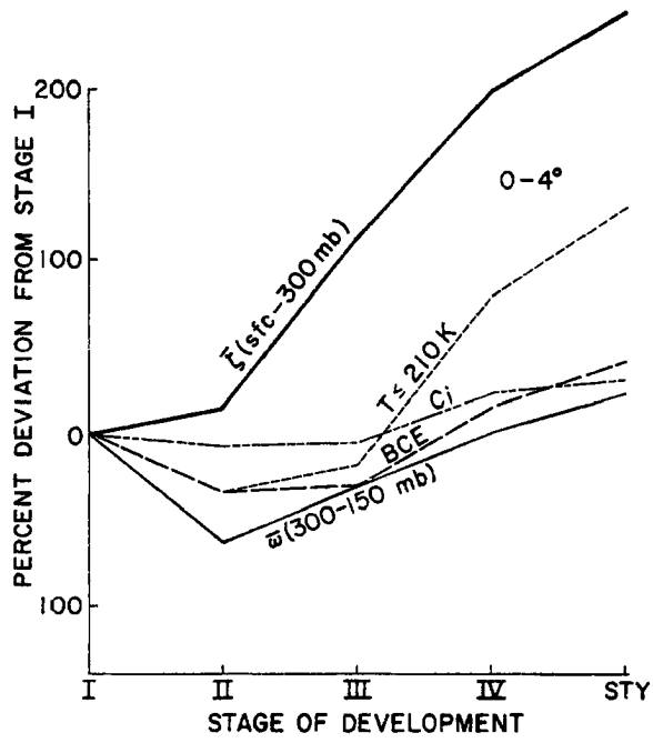
Fig. 57. Same as Fig. 56 except for r = 0-4^{\circ} .
