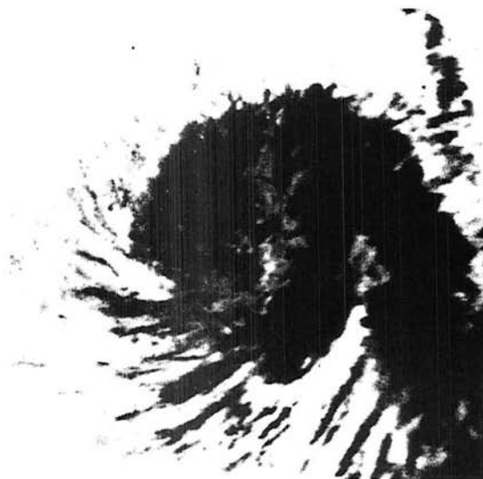
Fig. 29. Infrared picture of Fig. 27. Circulation center within the circle, 1 in = 484 km.
