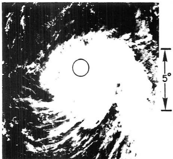
Fig. 27. Example of an embedded circulation center within the circle associated with a region of suppressed cloudiness. Developing cluster stage of Typhoon Pamela, 31 October 1972, 0222Z, 1 in = 484 km.
