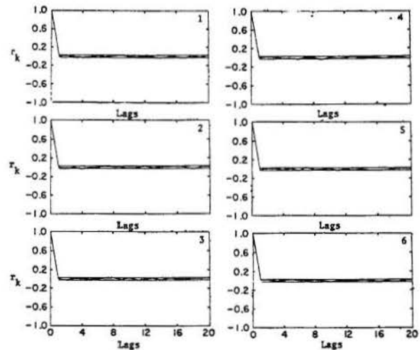
Fig. 4-1. Correlograms for the Six Generated Samples of Standard Normal Independent Variable, \xi_i , Used to Generate Study Samples. All Six Series of \xi_i are Serially Independent.
