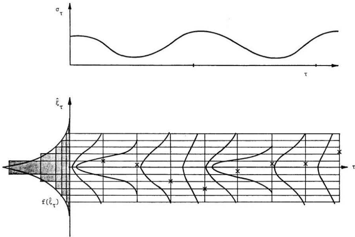
Figure 5-8. Illustration of the Effect of a Periodic Standard Deviation on the Distribution of the Estimated \hat{\xi}_i Component.
