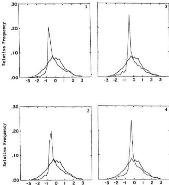
Fig. 5-6. Distribution of the X_i Series with Equal Amplitudes and Phases of the Harmonics in the Mean and Standard Deviation, and an Autoregressive Order-One Series, with \alpha_1 Allowed to Vary: (1) \alpha_1 = 0.2 , (2) \alpha_1 = 0.4 , (3) \alpha_1 = 0.6 , (4) \alpha_1 = 0.8 .
