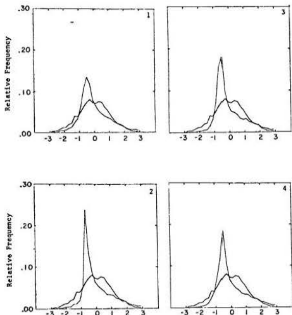
Fig. 5-3. Distribution of the \chi_i Series with Equal Amplitudes and Phases of Unremoved Harmonics in the Mean and Standard Deviation for: (1) P_m = 0.2 , (2) P_m = 0.4 , (3) P_m = 0.5 , (4) P_m = 0.6 .
