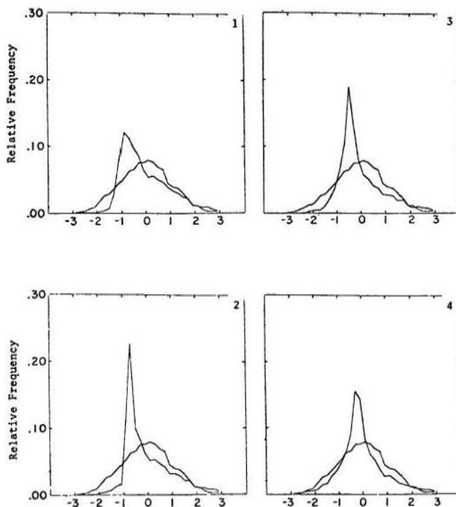
Fig. 5-4. Distribution of the \chi_i Series When the Amplitude of Unremoved Harmonics in the Mean are Held Constant ( P_m = 0.5 ), and the Amplitudes of the Unremoved Harmonics in the Standard Deviation are Allowed to Vary for: (1) C_s^2/C_m^2 = 0.25 , (2) C_s^2/C_m^2 = 0.667 , (3) C_s^2/C_m^2 = 1.50 , (4) C_s^2/C_m^2 = 4.00
